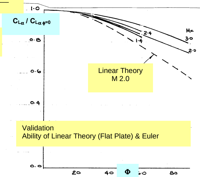
(b) Variation of Normalised C_{L\alpha} ( C_{L\alpha} / C_{L\alpha \phi=0} ) with \phi M varies
