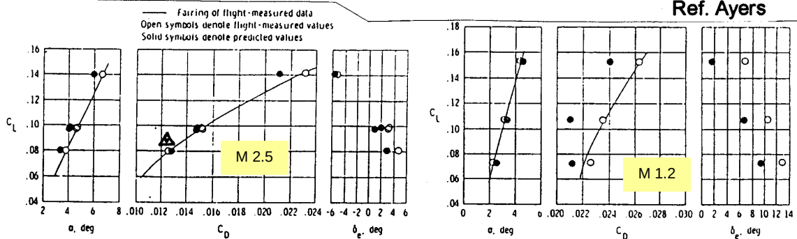
Fig. 4.3.3. XB-70 FLIGHT TEST DATA (Ref. Ayers & McCormick)
