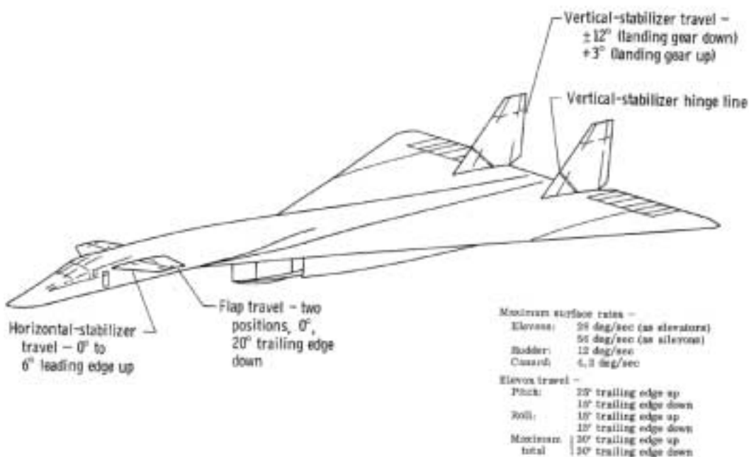
XB-70-1 Control Surface Movements
