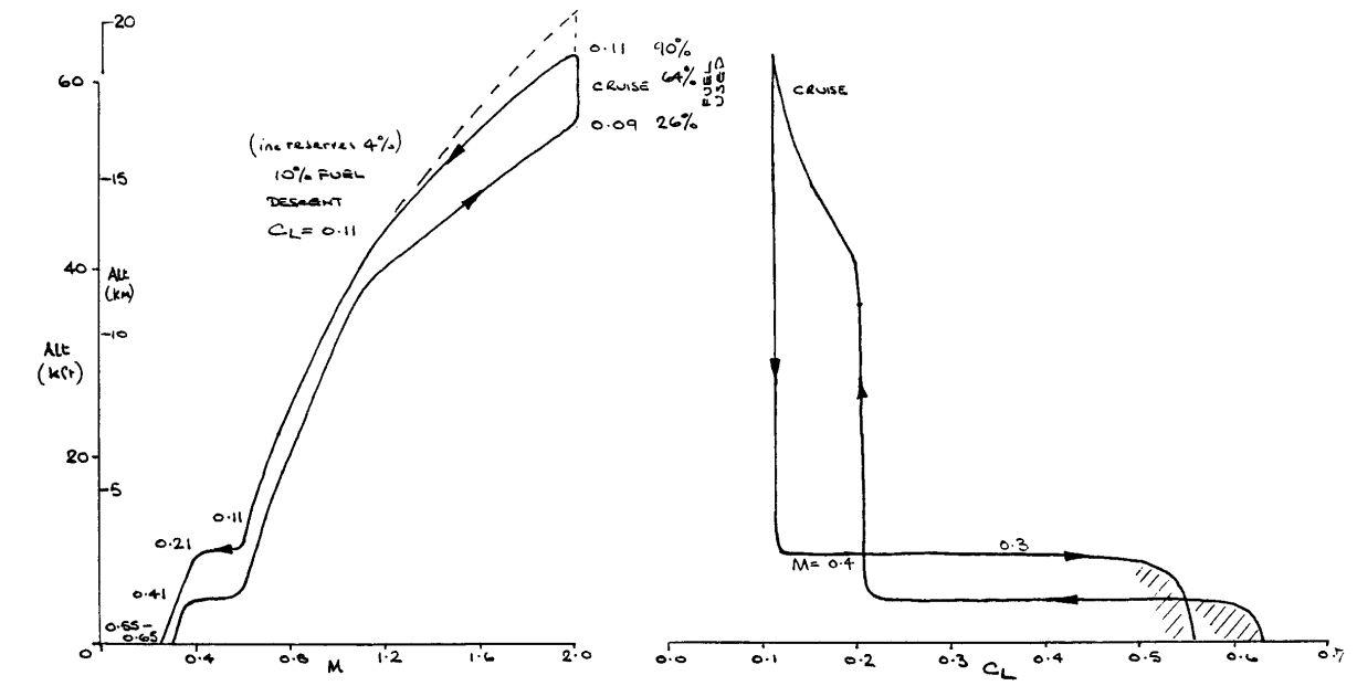
Fig.4.2.5. TYPICAL FLIGHT PROFILE SHOWING C_L VARIATION (McD Studies)
