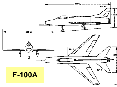
(a) Three-view drawing.
