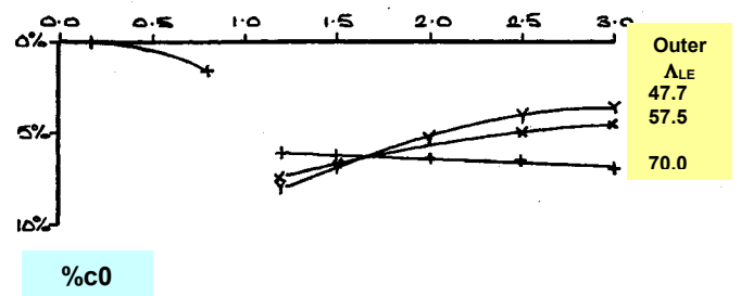
Fig.6.1.2. CRANKED PLANFORM SERIES, APEX LE SWEEP 65° & 70°, OUTER LE SWEEP VARIES LINEAR THEORY, EFFECT OF M ON C_{L\alpha} and \%C_0 MOVEMENT FROM LOW SPEED LOCATION
