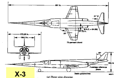
(a) Three view drawing.
