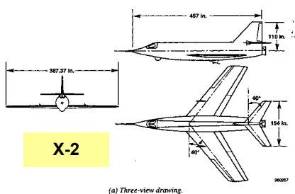
(a) Three-view drawing.
