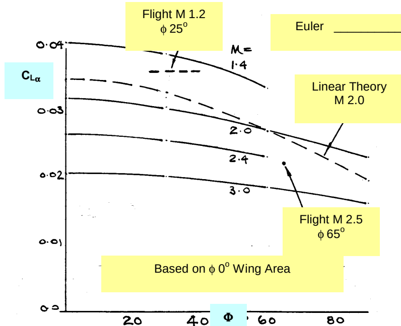
(a) Variation of C_{L\alpha} with \phi M varies
