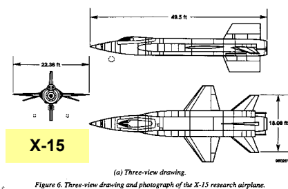
Figure 6. Three-view drawing and photograph of the X-15 research airplane.
