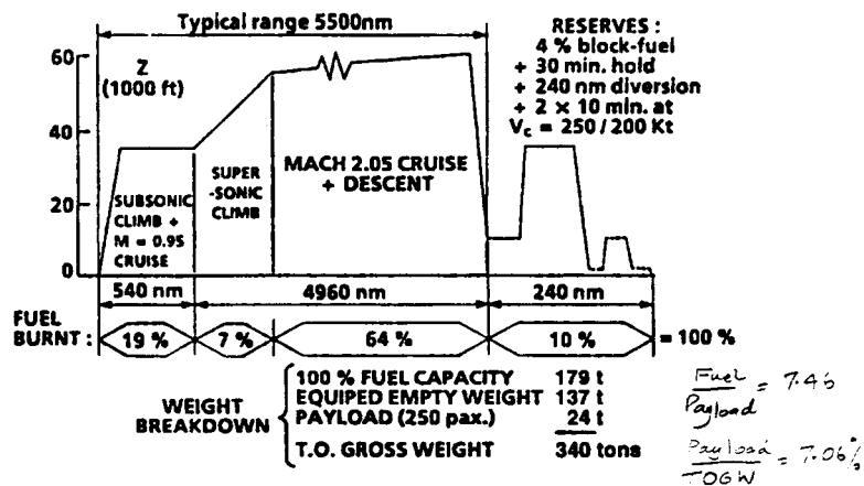
Fig. 4.2.7. FUEL WEIGHT BREAKDOWN FOR 5500 NM FLIGHT Ref. Thibert
