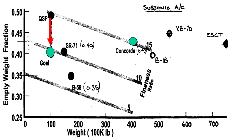
(c) OEW/MTOW - TOW
