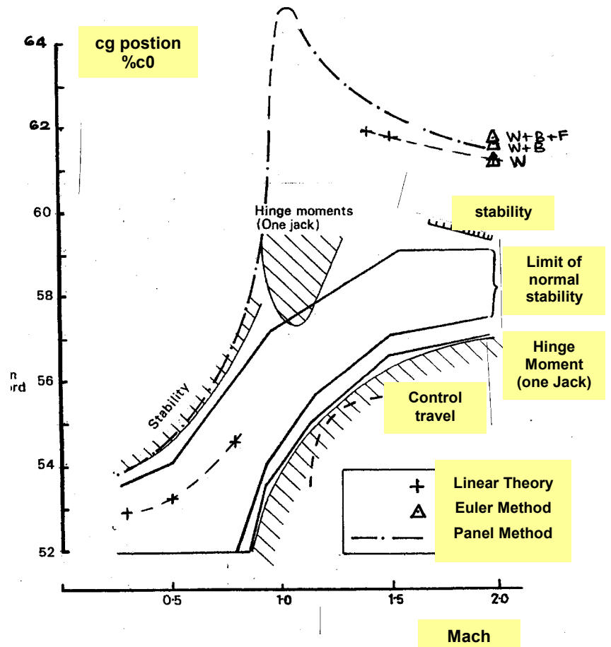
(b) Centre of Gravity Location ( \%c_0 ) and Centre of Pressure Variation with M
