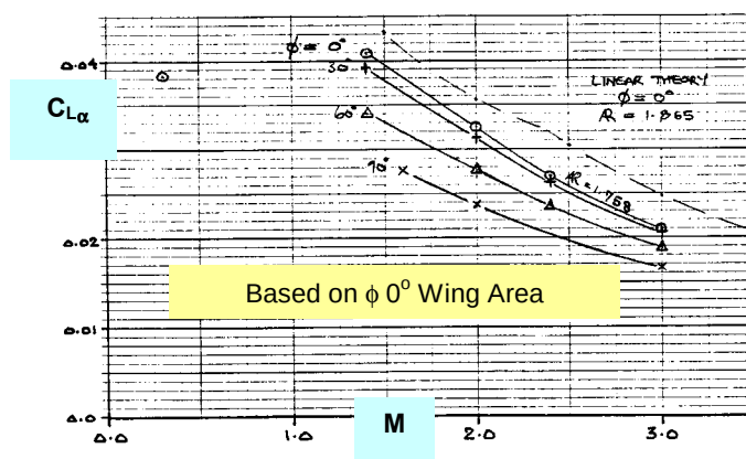
(d) XB-70 Wing, Variation of C_{L\alpha} with M Tip Fold Angle varies
