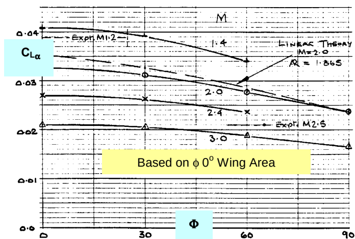
(c) XB-70 Wing, Variation of C_{L\alpha} with Tip Fold Angle M varies
