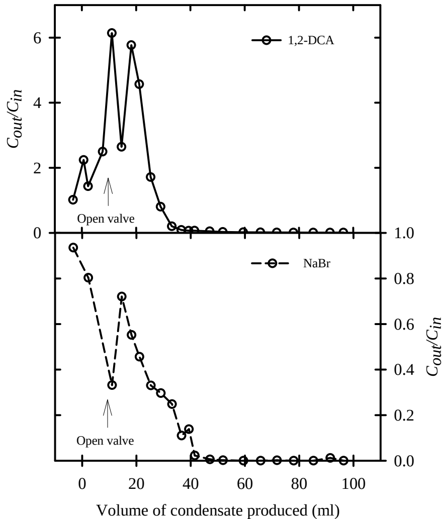
Figure 3.7. Relative concentration of 1,2-DCA and NaBr in condensate produced during heating experiment.
