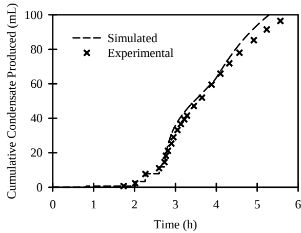
Figure 5.9. Simulated and experimentally determined cumulative condensate produced.
