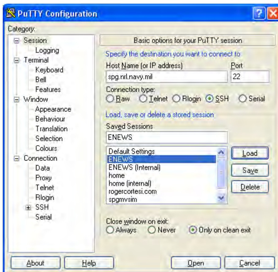
Step 1: configure for connecting to spg.nrl.navy.mil on port 22
