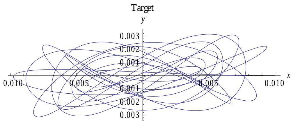
Figure 4.10. Displacement plots for free vibration, damped unequal stiffnesses, no added discrete masses with initial condition of u_0(0) = 0.01 \text{ ft} with \alpha = 0.0007812 , \beta = 0.0007812
