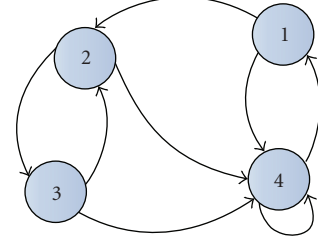
FIGURE 1: A directed graph.
