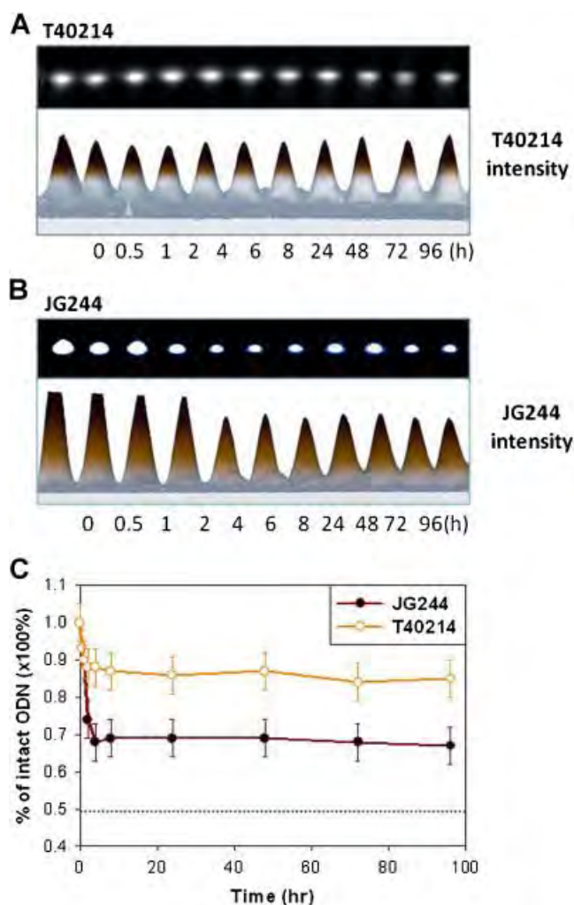
Fig. 3. Nuclease resistance assays. The gel shows how the intensities of T40214 (A) and JG244 (B) varied with time from 0 to 96 hr in serum. C: Plot of % of intact ODN versus time provides the pharmacokinetic information on T40214 and JG244 in serum.
