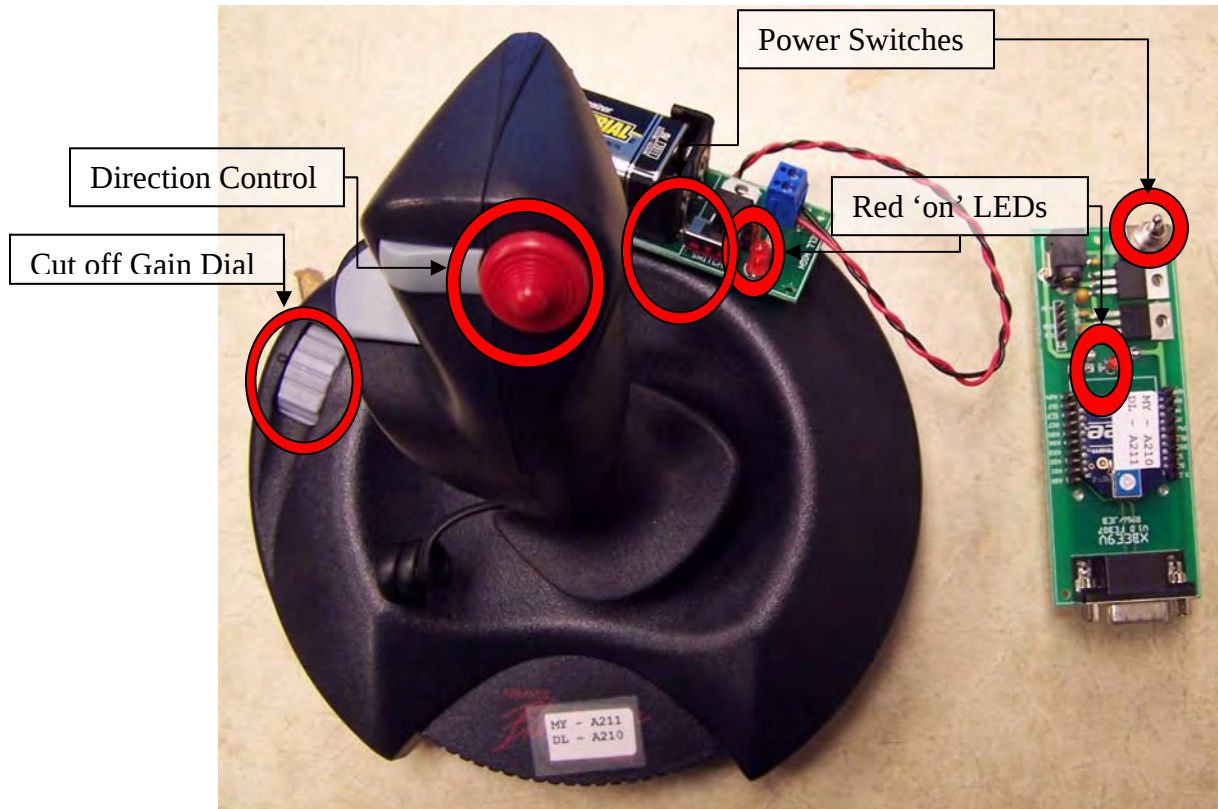
Figure B-3. Picture of the RC joystick and the Xbee transceiver.
