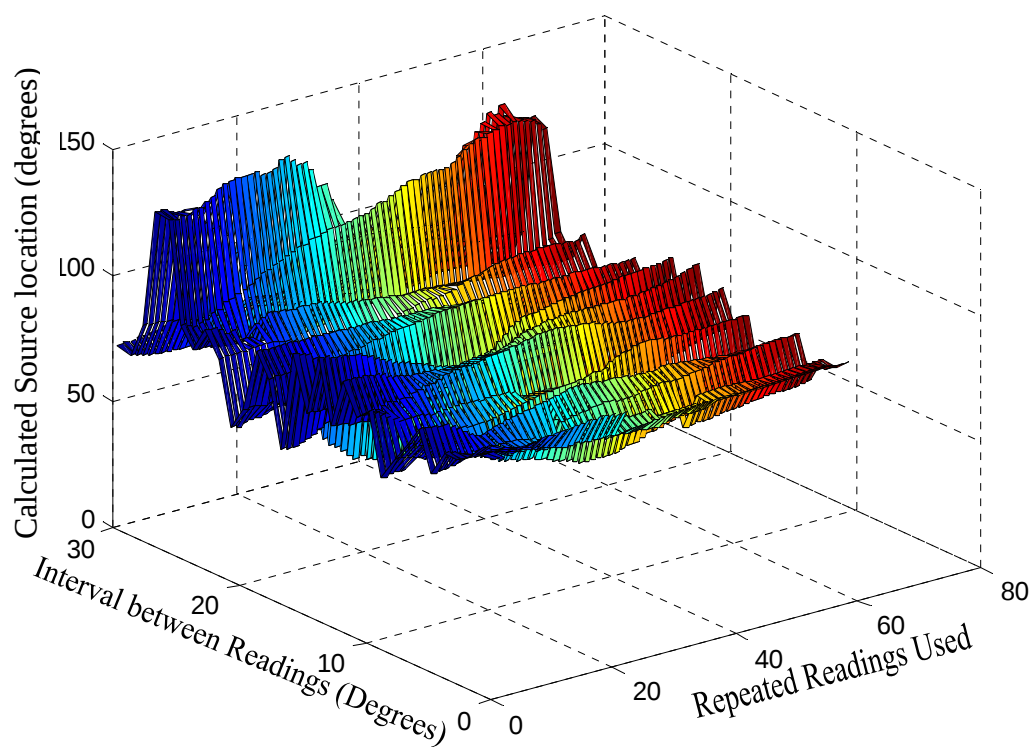
Figure 3-14. Plot of source location versus degree interval and repeats, ribbons repeats.
