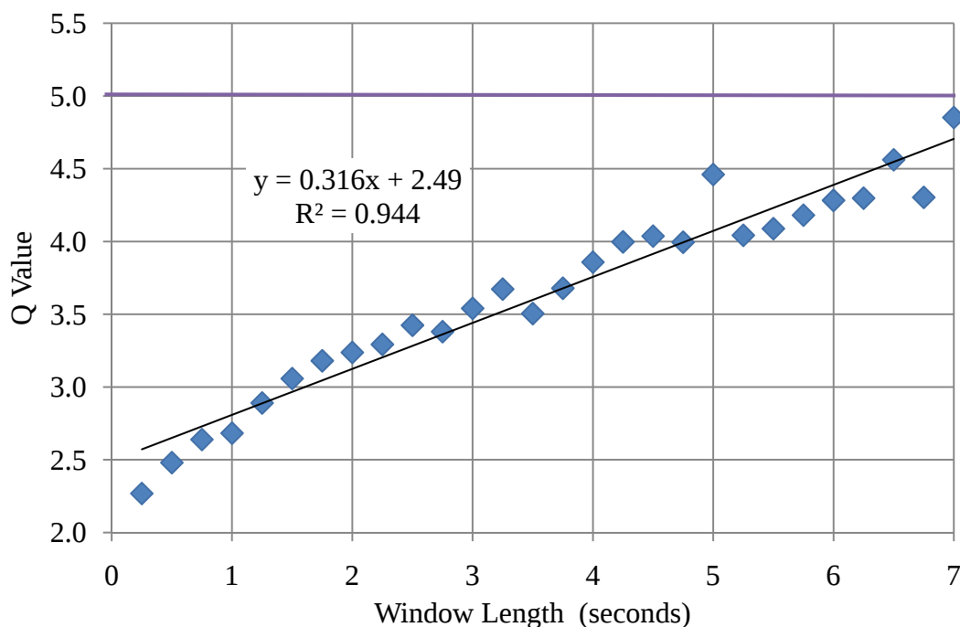
Figure 3-3. Relationship of Q value versus window length when Q < 5 .
