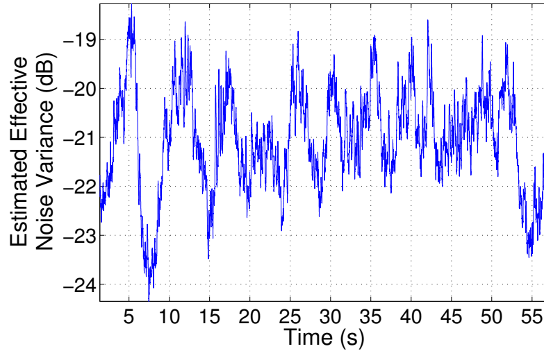
Figure 3.6.2: Top-left element of the estimated effective noise correlation matrix, [\hat{\mathbf{R}}_{\mu}]_{(1,1)} , from October 26, 2008 at time 0800. The variance is tracked using an exponential window algorithm.. This value is a measure of the effective noise variance. Over the one minute packet there is a 5 dB peak to peak change with a coherence time of approximately five seconds.
