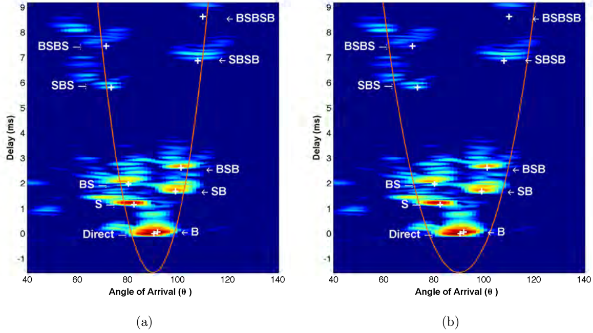
Figure 4.5.2: Arrivals from SPACE08 data during calm weather conditions. The orange line specifies the delay calculated for the time-aligned uniform beam weights. Figure (a) shows the bounds for \alpha_b = 1 and figure (b) with \alpha_b = \frac{1}{2} .
