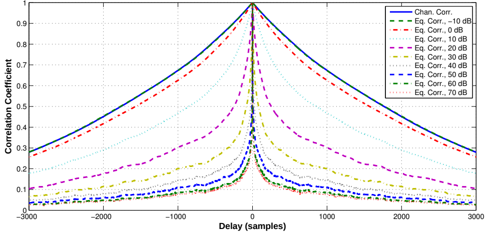
Figure 6.7.1: The correlation of a single-coefficient Markov channel with a correlation window of N_{\text{win}} = 2400 symbols. There is a smooth transition from the channel correlation down to a minimum correlation as the SNR increases.
