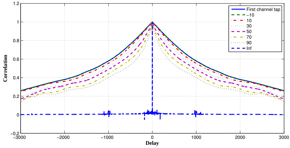
Figure 6.7.6: Correlation function for the first coefficient of the channel and the first coefficient of the equalizer for several SNR values. Notice that there is a smooth transition from the correlation of the channel down to the 90dB. This trend continues as the SNR continues to be increased (not shown). The transition to the no-noise correlation levels happens at much higher SNR than for the single coefficient channel (shown in the figure at 200dB).
