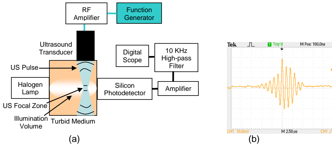
Figure 3a) Experimental set-up for AO measurements of ultrasound-modulated incoherent light. 3b) Optical modulation at 1 MHz detected and recorded on the digital scope.
