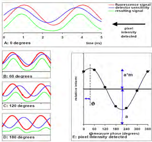
Figure 5. Cross-Correlation Principle
