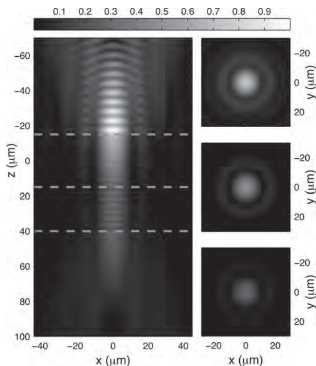
Figure 5. The focused field magnitude |E(x, y, z)| for \bar{\nu} = 1000 \text{ cm}^{-1} (a free space wavelength of 10 \text{ μm} ), the four-layer object of Figure 2 and the angular planewave spectrum of Figure 4d–f plotted on a normalized scale. The free space focal plane is at z^{(0)} = 0 . One transverse–axial ( x – z ) section is plotted at y = 0 and three transverse–transverse ( x – y ) sections are plotted at z = -15 \text{ μm} , z = 0 , and z = 15 \text{ μm} . In this example, the Cassegrain pupil is filled, i.e., there are no apertures limiting the width of the illuminating beam before the focusing optics.
