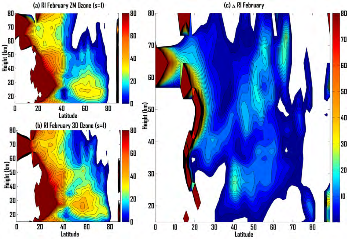
Figure 3. Monthly averaged refractive index squared (RI) in February for: (a) ZMO3 for planetary wave s=1 ; (b) 3DO3 for planetary wave s=1 ; and (c) difference in RI ( \Delta\text{RI} = 3\text{DO3} \text{ minus } \text{ZMO3} ). Regions of wave evanescence ( \text{RI} < 0 ) are depicted by regions without shading (white). In all plots, the RI has been multiplied by \alpha^2 ; the contour interval is 4.
