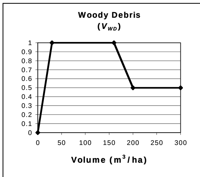
Figure 19. Relationship between woody debris and functional capacity.
