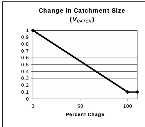
Figure 5. Change in effective size of the wetland catchment (V CATCH ) and functional capacity.
