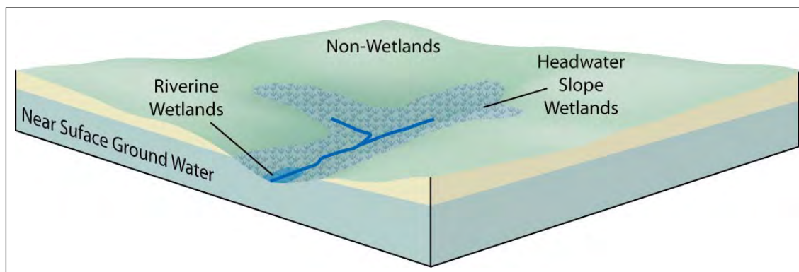
Figure 4. Generalized landscape position of Headwater Slope wetlands in the Coastal Plain of South Carolina.
