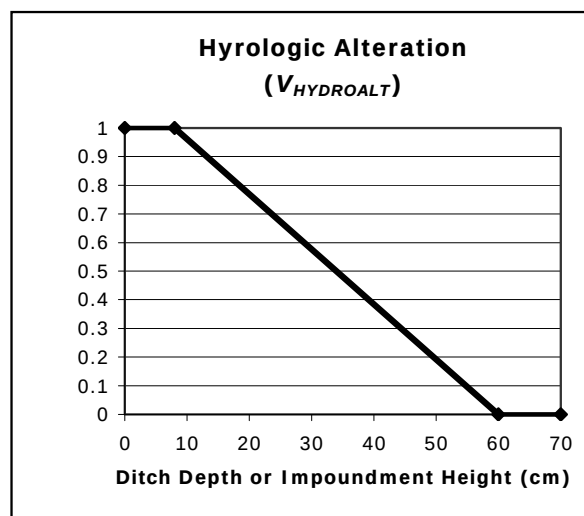
Figure 10. Relationship between depth or height of drainage or impoundment ( V_{HYDROALT} ) and functional capacity.
