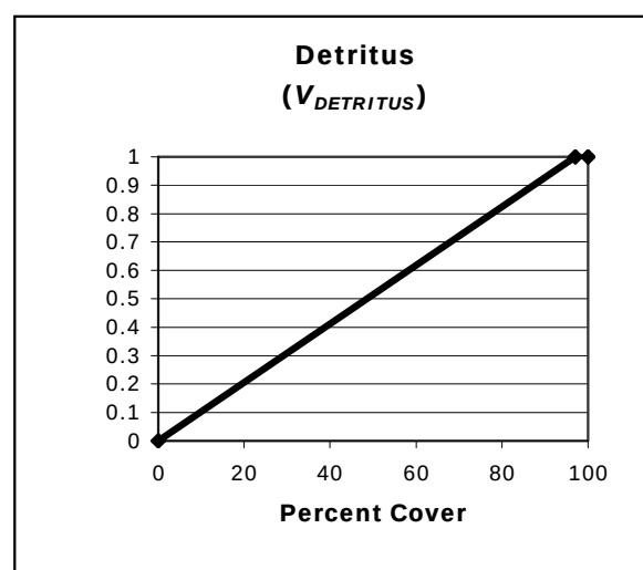
Figure 18. Relationship between average percent cover of detritus ( V_{DETRITUS} ) and functional capacity.
