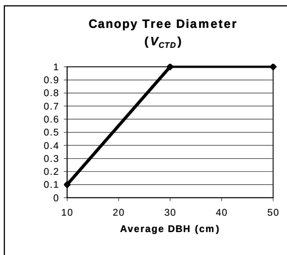
Figure 12. Relationship between average canopy tree diameter ( V_{CTD} ) at breast height and functional capacity.
