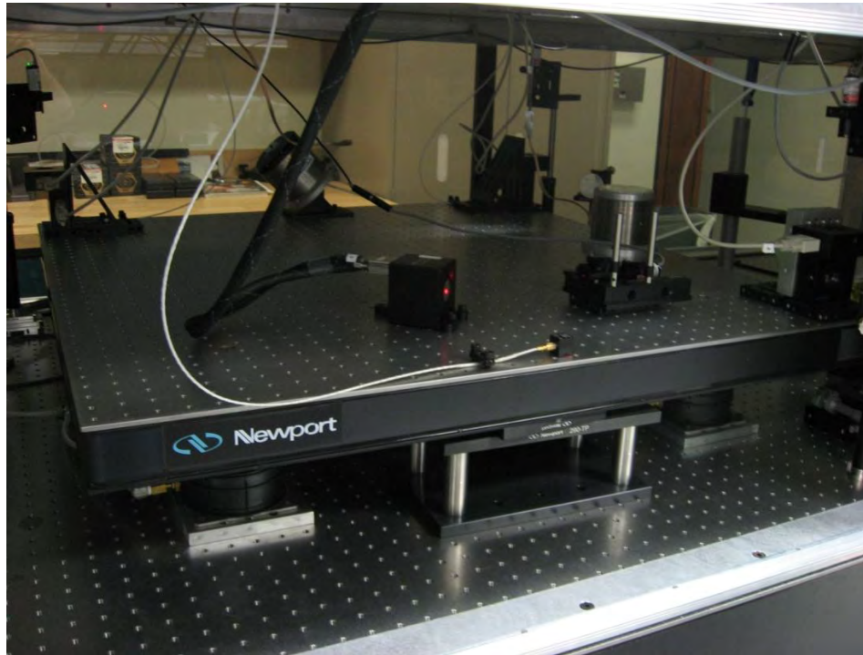
Figure 5. Experimental Configuration
