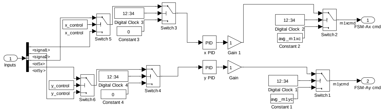
Figure 15. PI Controller
