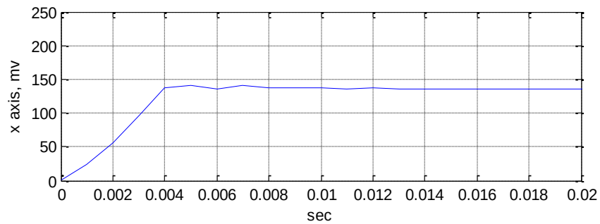
Figure 9. Mirror Position before Critical Gains
