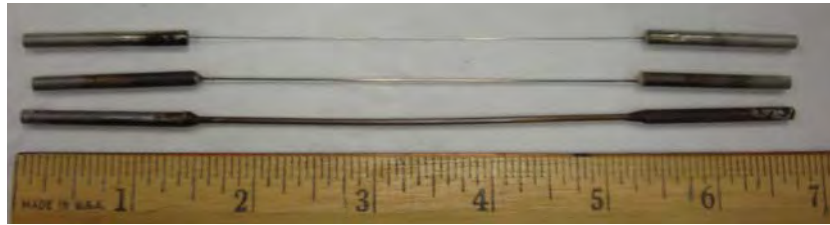
Figure 2.1: Image of 100, top, 250 and 1100, bottom, Micron Diameter Test Sections
