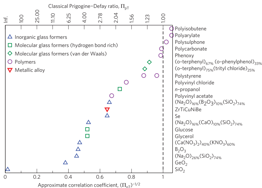
Figure 3 | Literature values of the classical (NpT) Prigogine-Defay (PD) ratios \Pi_{pT}^{\text{classical}} of 22 glass formers. The liquids, which are sorted according to reported value of the PD ratio, include inorganic glass formers (triangles pointing up), hydrogen-bond-rich molecular liquids (squares), van der Waals molecular liquids (diamonds), polymers (circles), and a metallic alloy (triangle pointing down). The inverse square root of the classical NpT Prigogine-Defay ratio gives an estimate for the correlation coefficient (lower x-axis). Strong correlations are found in van der Waals bonded molecular liquids and polymers (the Supplementary Information provides the PD values shown in the figure and relevant references; note that each symbol in the figure corresponds to the liquid listed to the right).
