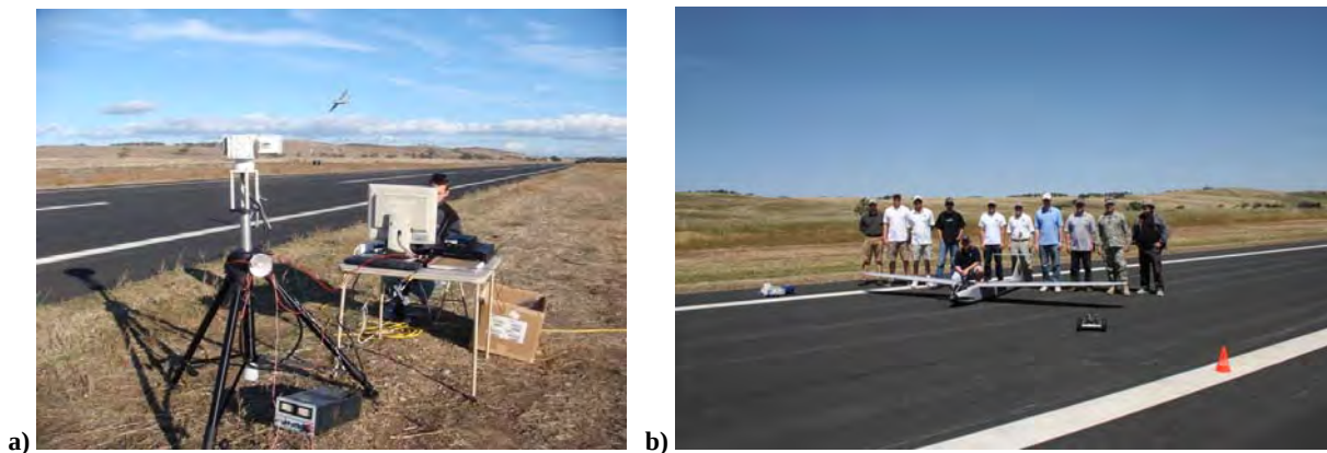
Figure 17. Snowflake ADS / T-20 UAV tracking station (a) and a Blizzard team with the Camp Roberts Base Commander (b).
