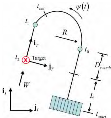
Fig. 2 Terminal guidance manoeuvre
