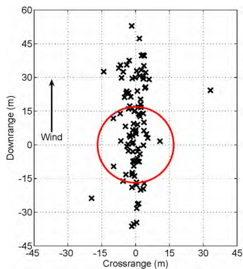
Fig. 9 Monte Carlo simulation dispersion
