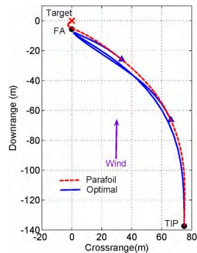
Fig. 8 Optimal real-dynamics-augmented guidance for W = -7.7 m/s (▲ trajectory update)
