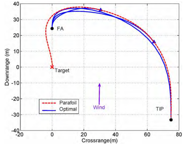
Fig. 7 Optimal real-dynamics-augmented guidance for W = -3.7 m/s (▲ trajectory update)
