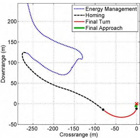
Fig. 10 Test results of precision placement algorithm
