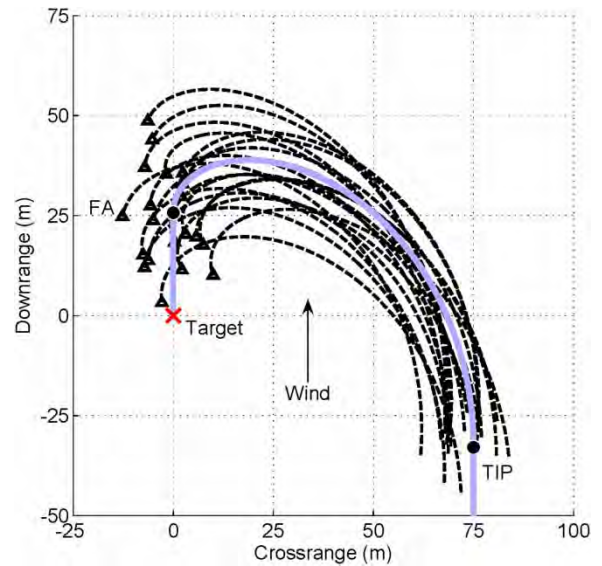
Fig. 4 Final turn trajectories with initial condition errors
