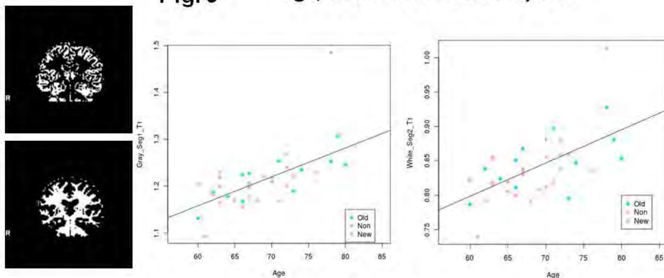
Fig. 9 QT_1 Analysis: T1 increases with age, but is not affected by ADT
