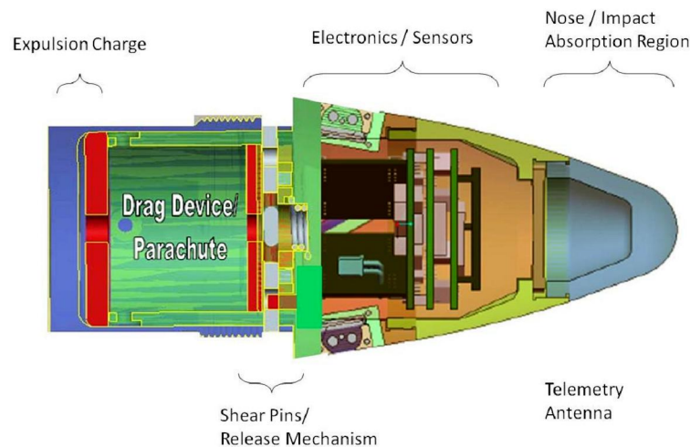
Figure 5. Preliminary system geometry.
