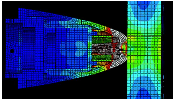
Figure 8. The FEA model of crushable nose design on Reuse-Fuze.
