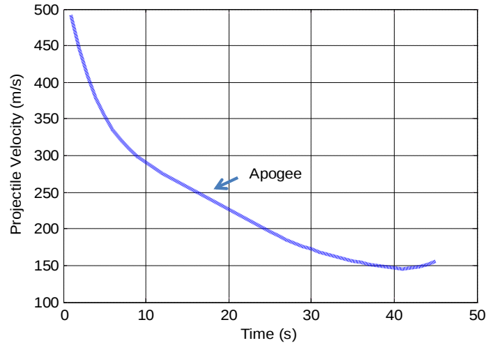
Figure 4. Typical deceleration profile of a 155 mm projectile.
