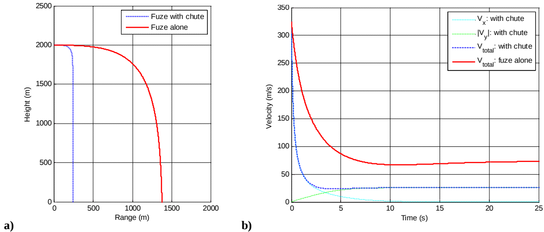
Figure 7. Fuze trajectory after expulsion (a) and deceleration profile (b).
