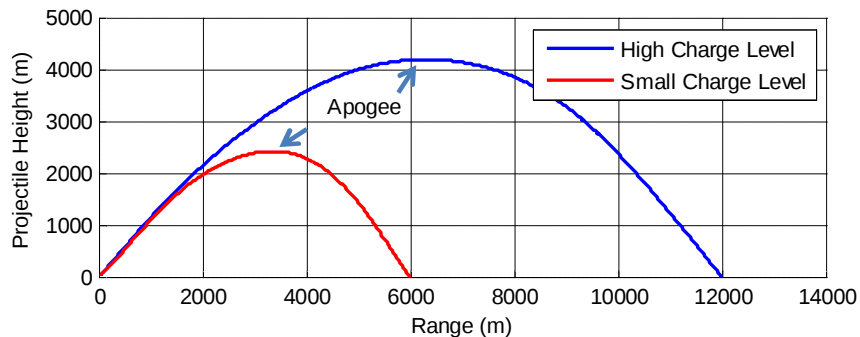
Figure 3. Example of 155 mm projectile trajectories at different charge levels (with 50^\circ QE).
