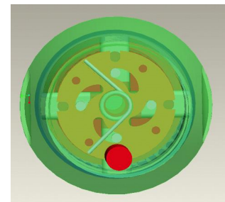
Figure 9. Mechanical release system (fuze cross section).
