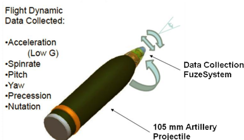
Figure 1. Fuze data collection system.
