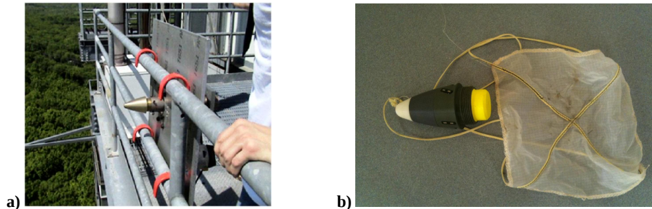
Figure 6. Spinning ejection test system at Picatinny Arsenal (a) and a drogue parachute (b).
