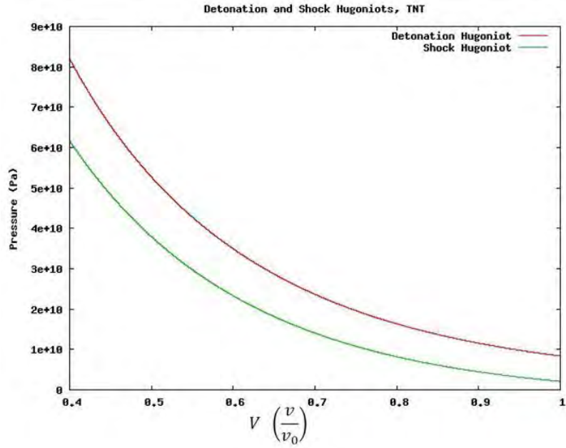
Figure 3: Detonation and Shock Hugoniot for TNT using the JWL Equation of State
