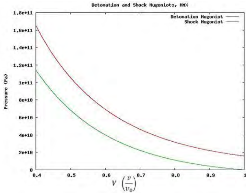
Figure 4: Detonation and Shock Hugoniot for HMX using the JWL Equation of State
