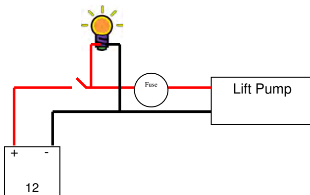
Figure 62: Wiring Schematic for the Lift Pump
