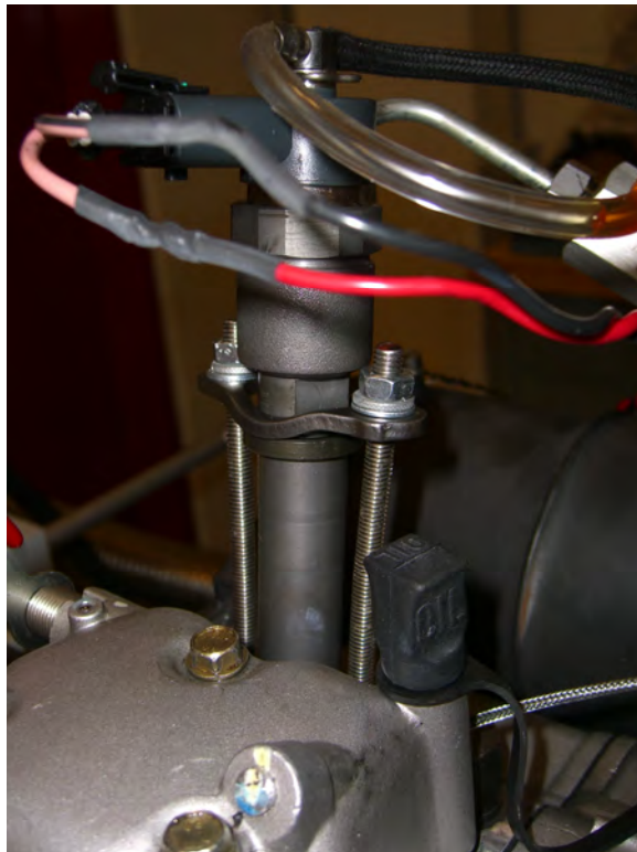
Figure 57: Bosch Solenoid Injector
