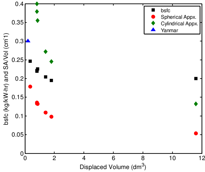
Figure 2: Best-Minimum BSFC Data for a Range of Engine Sizes, Including the Current Yanmar L48V. Also Shown are Analytic Results of Surface Area to Volume of These Engines Assuming Both a Spherical and Cylindrical Combustion Chamber
