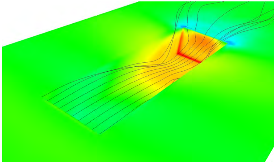
Figure 24. Flow Visualization of the Empty Bay from CFD
