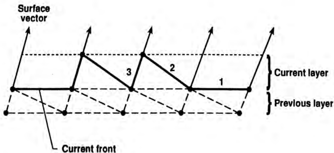
Figure 10. Advancing layers propagation method 6
