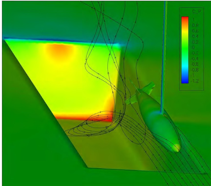
Figure 16. Pressure Distribution of Cavity and Store generated with USM3D
