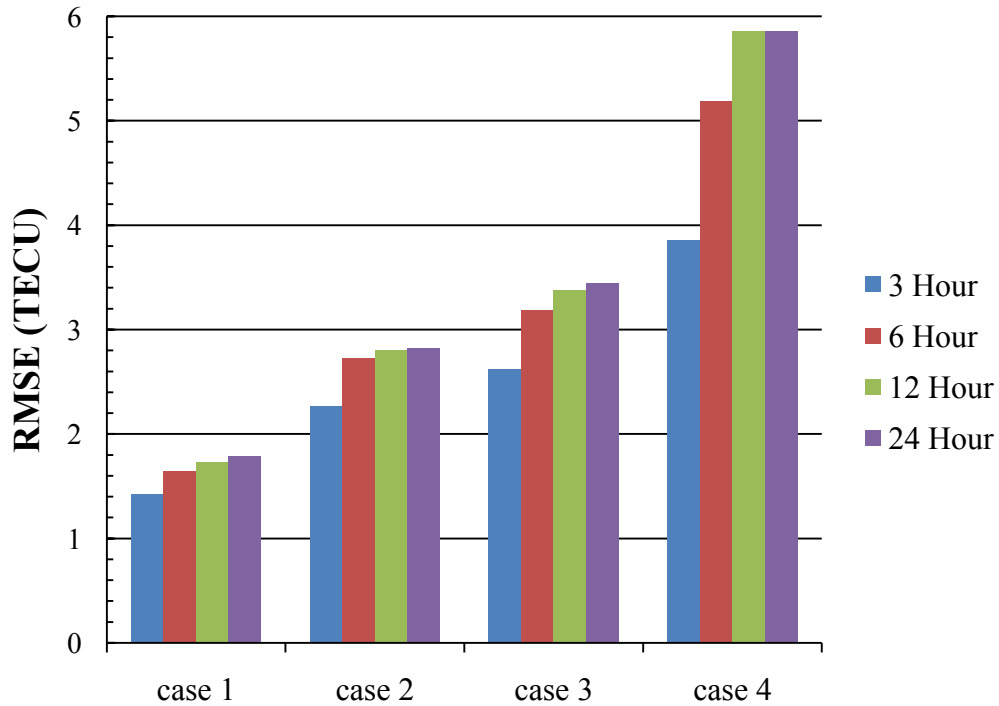
(b) RMSE
