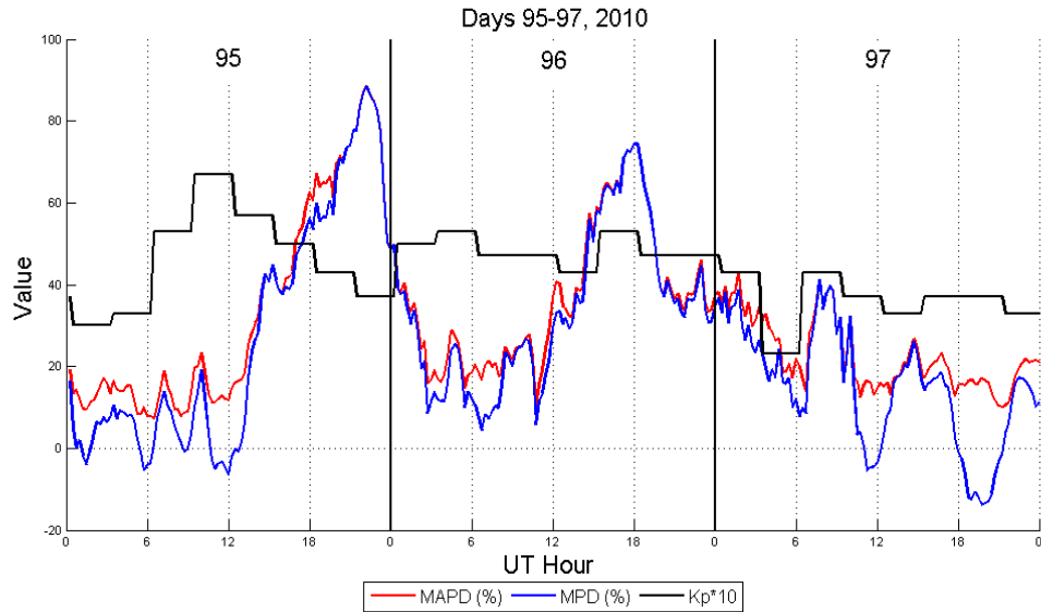
Figure 19. MPD and MAPD for case 3, days 95-97, 2010. Note the peak MAPD of 88% on day 95. Nighttime MDP (0215UT-0900UT) values decrease, but are not necessarily negative as they were for cases 1 and 2.
