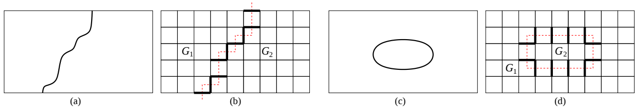
Figure 1: Image segmentation and graph cuts. (a) An image segmented by an open boundary. (b) The graph model for (a) and the graph cut for its segmentation boundary. (c) An image segmented by a closed boundary. (d) The graph model for (c) and the graph cut for its segmentation boundary.
