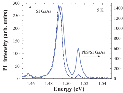
FIG. 5. (Color online) Comparison of the 5 K PL in the near infrared range of the SI GaAs substrate and the PbS/GaAs sample. The spectra are shown in the same arbitrary units.
