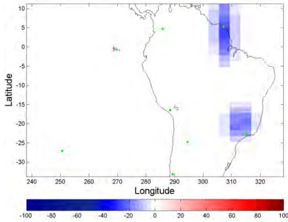
(a) 00UT
