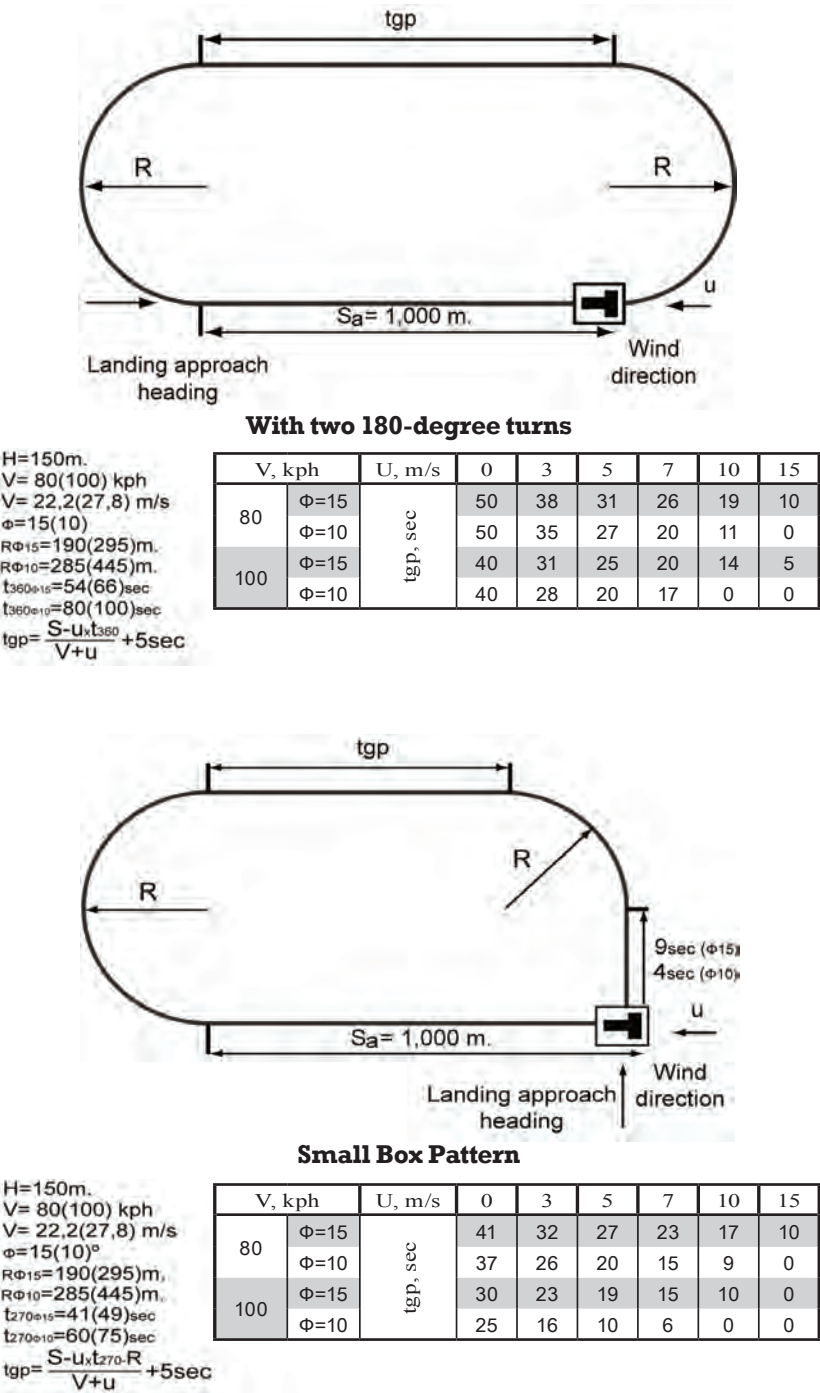
Figure 8. Methods of approach to a site depending on wind direction.
