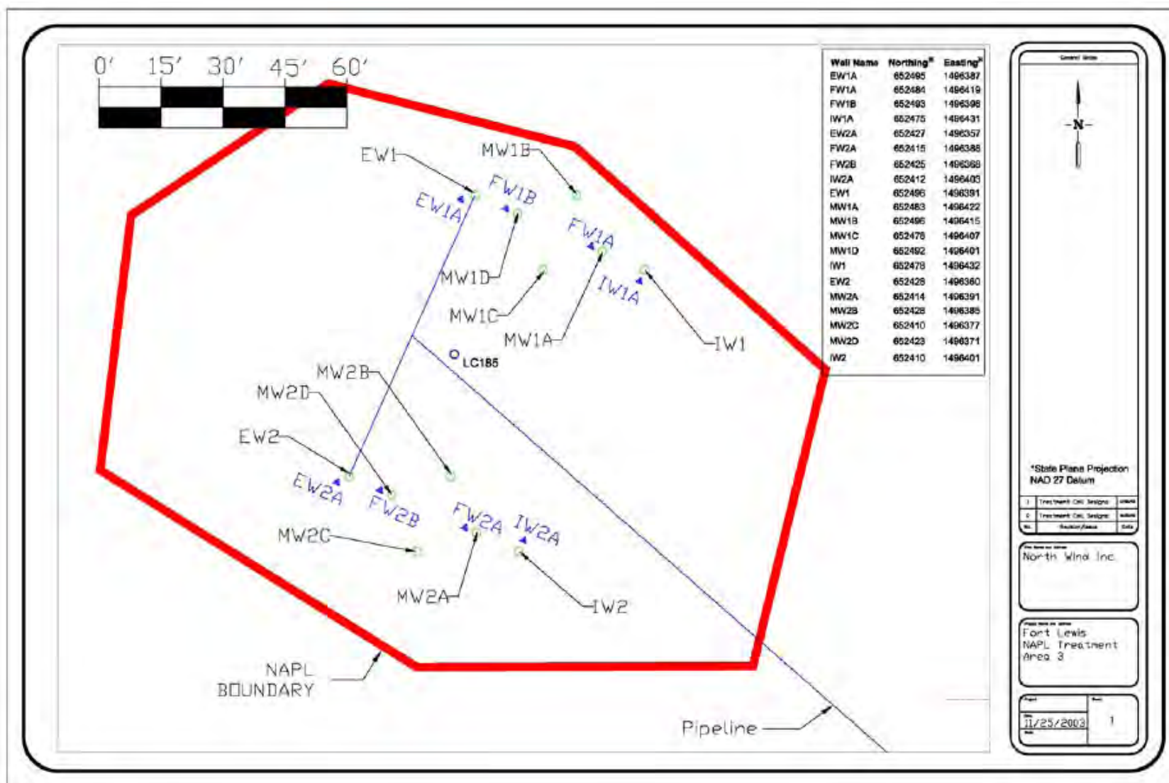
Figure 5-2. Well Locations within Treatment Cells at Ft. Lewis EGDY.
