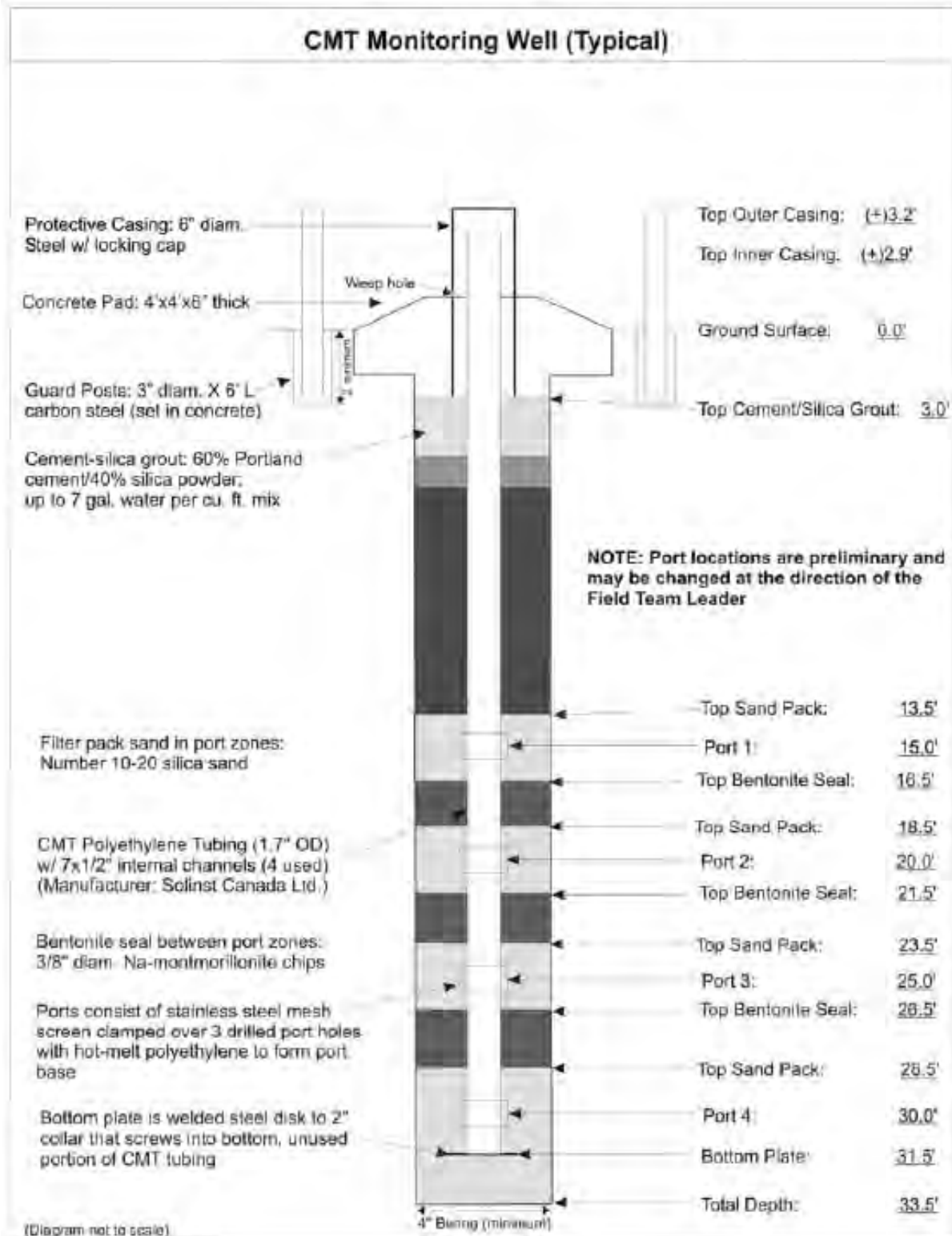
Figure 2-1. Typical CMT Monitoring Well Configuration.
