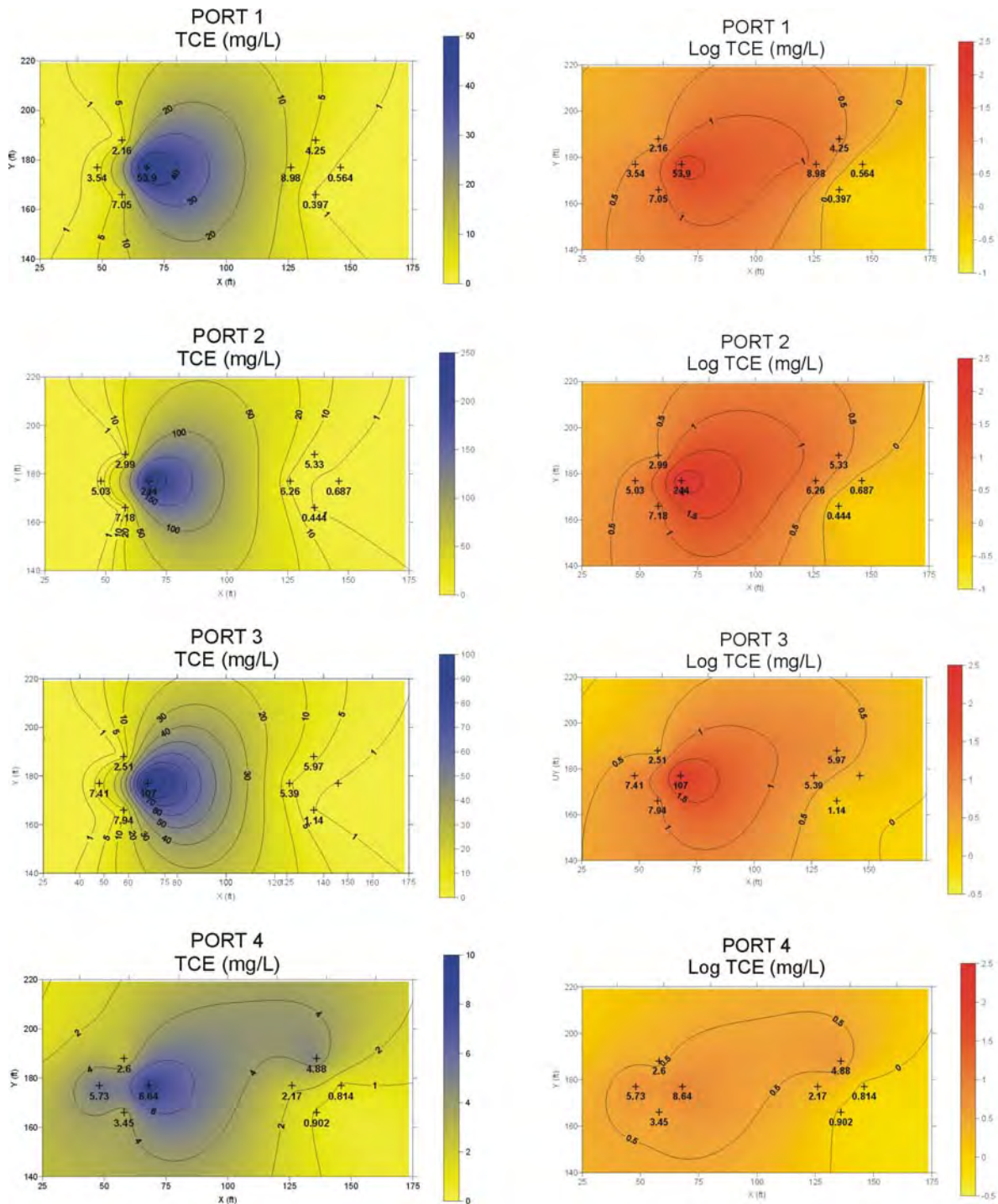
Figure 5-6. Distribution of TCE in Groundwater Within Two Treatment Cells at Four CMT Depth Intervals: 13-14 ft bgs (Port 1), 18-19 ft bgs (Port 2), 23-24 ft bgs (Port 3), and 28-29 ft bgs (Port 4) During Phase 1 Sampling.
