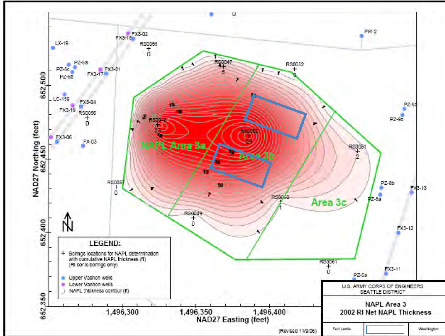
Figure 4-3. Inference of NAPL Distribution Within NAPL Area 3 Based on Data Gathered During the Phase 2 RI (2002) (USACE, 2008). Boxes Highlighted in Blue Indicate Target Treatment Cell Locations.
