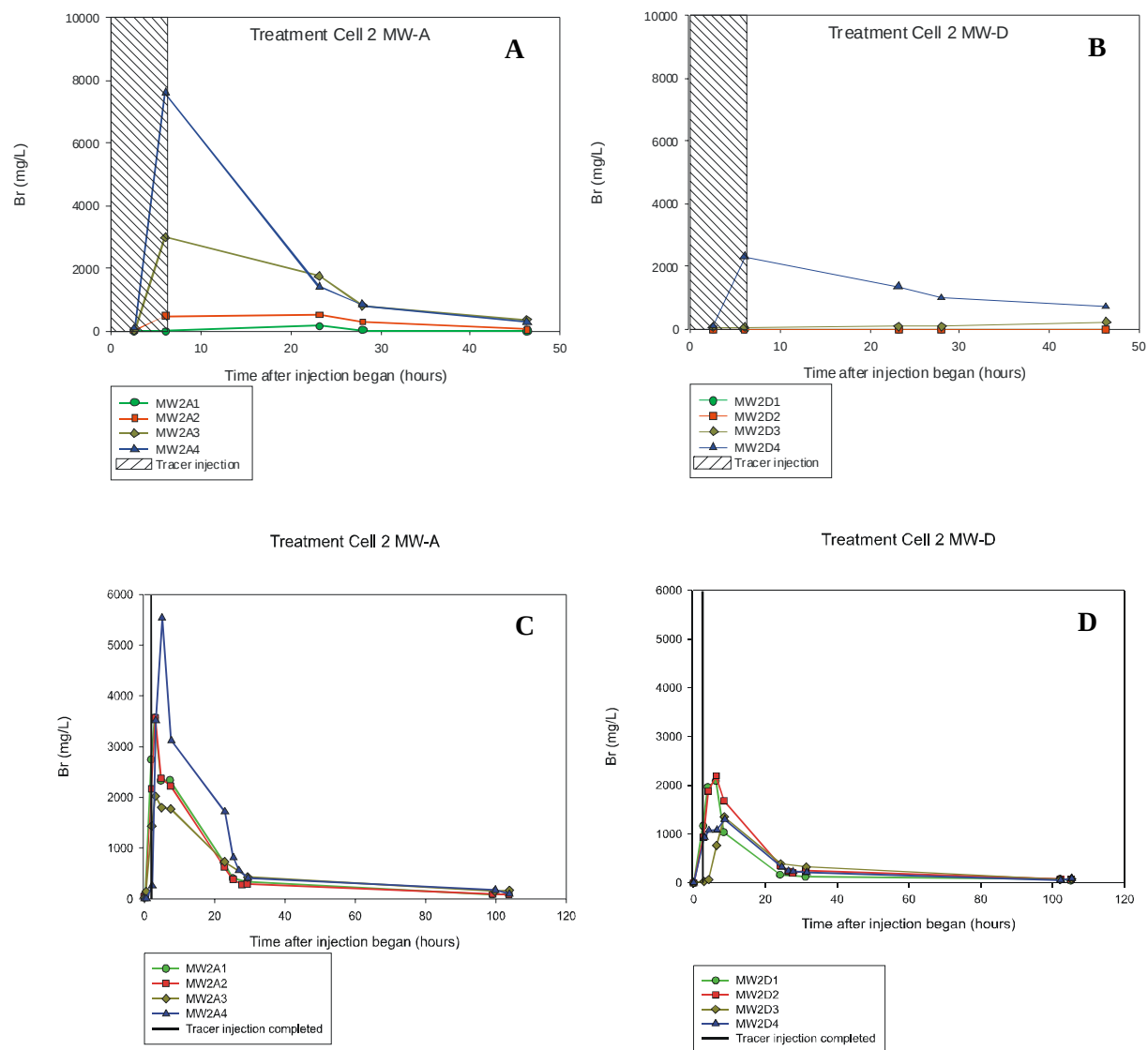
Figure 5-5. Comparison of Vertical Distribution of Tracer in Monitoring Wells A and D in Treatment Cell 2 Following Bromide Injections in the Original (A and B) and New (C and D) Injection Wells.
