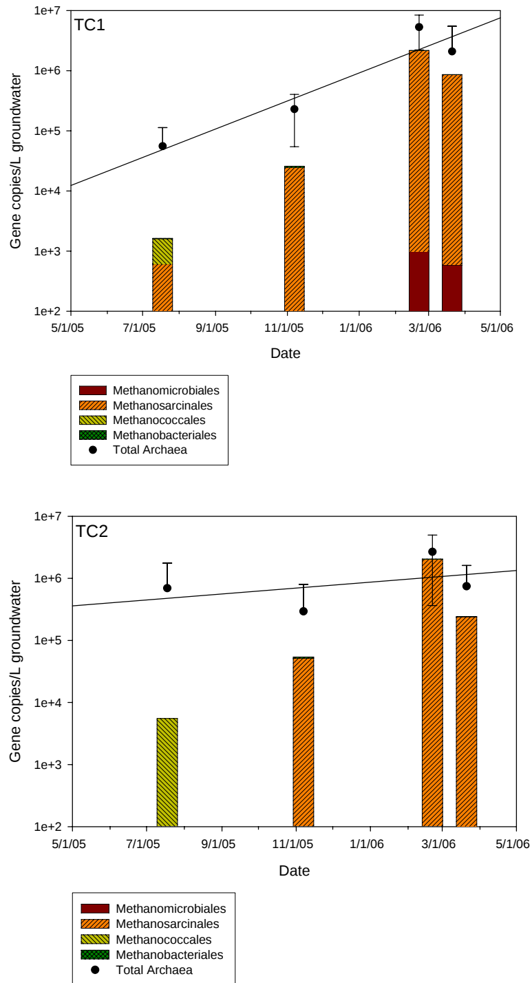
Figure 5-29. Response of Methanogenic Populations (order level) Using qPCR During Phase 3 Operations, Values Represent the Mean of n=4 (Port 4 of each CMT well) Sampling Points for Each Treatment Cell.
