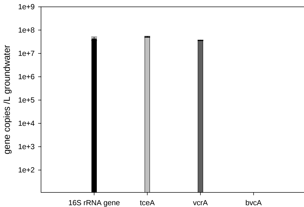
Figure 5-23. qPCR Results of Bioaugmentation Culture used at NAPL Area 3.
