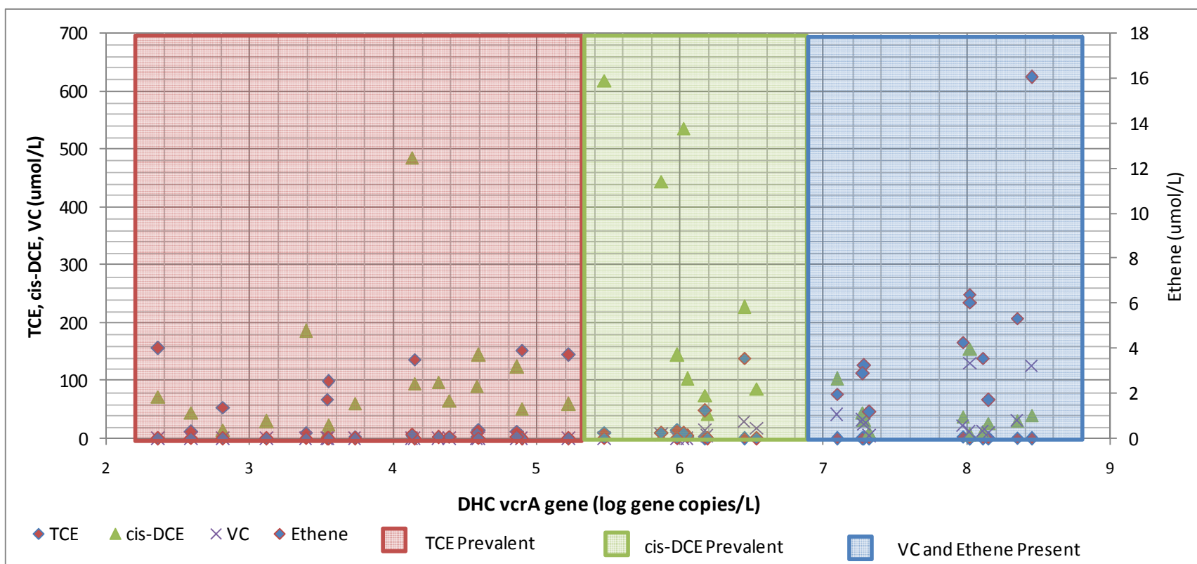
Figure 5-26. Relationship Between TCE and Reductive Daughter Products and Concentrations of DHC vcrA Genes.
