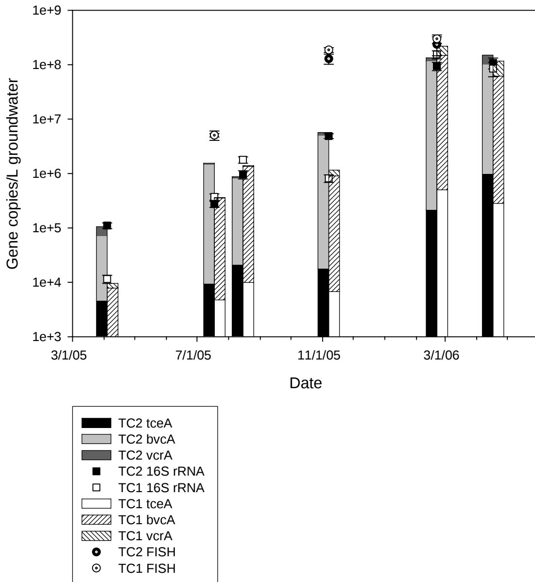
Figure 5-22. Summary of DHC qPCR Results for the 16S rRNA, bvcA , vcrA , and tceA Genes as the Mean (n=4) for Each Treatment Cell and FISH Results Targeting the 16S rRNA Gene.
