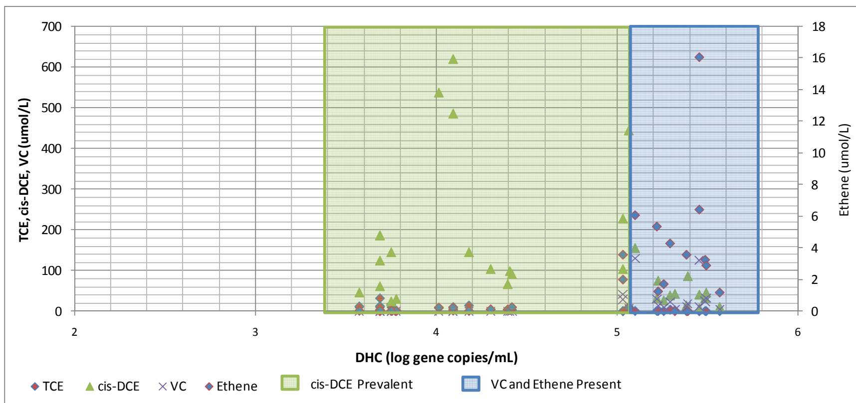
Figure 5-28. Relationship Between TCE and Reductive Daughter Products and Concentrations of Active DHC Cells.
