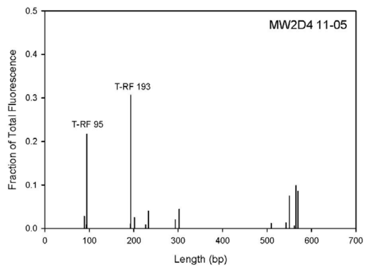
Figure 5-21. T-RFLP Response in Bacteria During Phase 3 in MW2D4.
