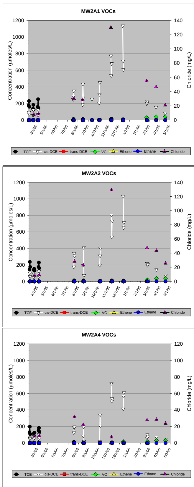
Figure 5-12. Molar Mass Plots of TCE and Reductive Daughter Products During Phases 2 and 3 of the Demonstration at MWA in Treatment Cell 2.
