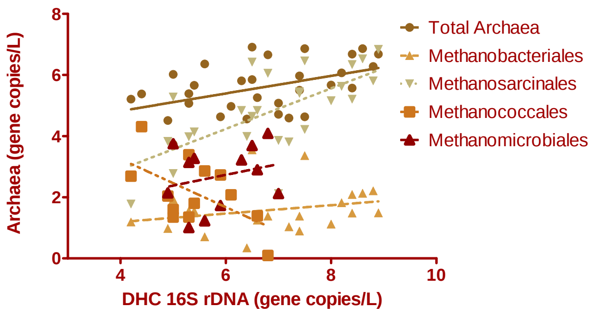
Figure 5-30. Relationship Between Methanogenic Orders and DHC Concentrations Measured using qPCR in Both Treatment Cells.
