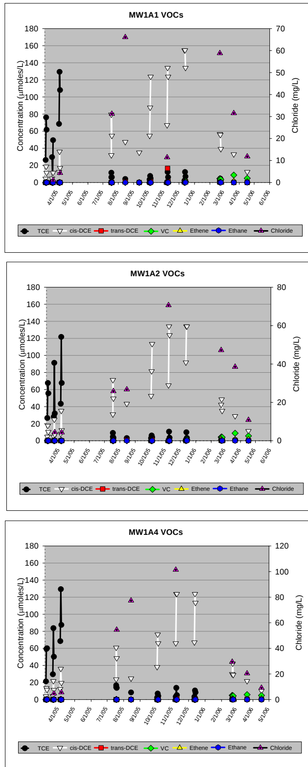
Figure 5-10. Molar Mass Plots of TCE and Reductive Daughter Products During Phases 2 and 3 of the Demonstration at MWA in Treatment Cell 1. Vertical Lines Illustrate Samples Collected Before, During, and After a Recirculation or Injection Event.
