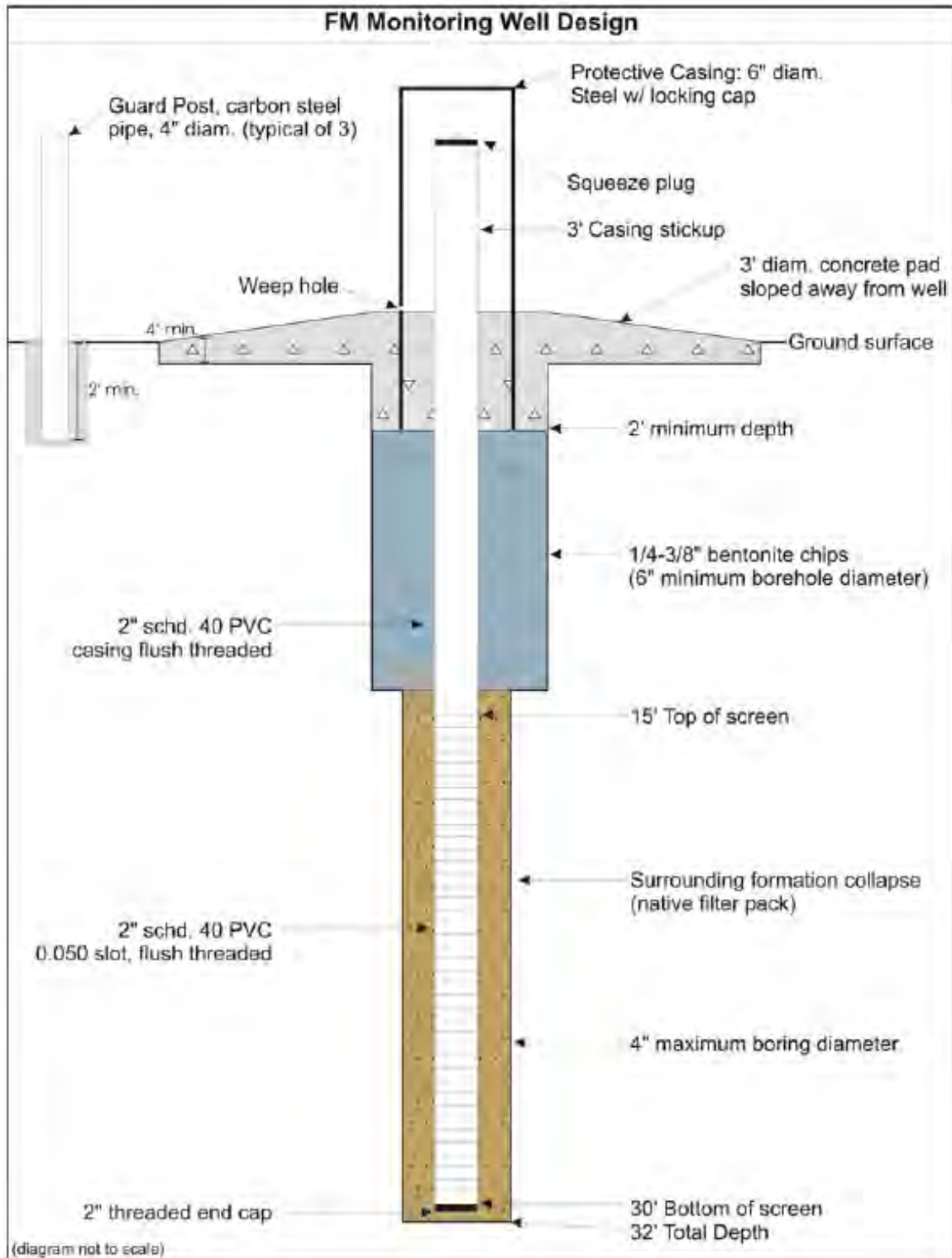
Figure 5-4. Example PFM Well Design.
