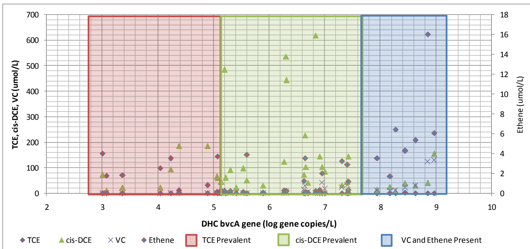
Figure 5-25. Relationship Between TCE and Reductive Daughter Products and Concentrations of DHC bvcA Genes.
