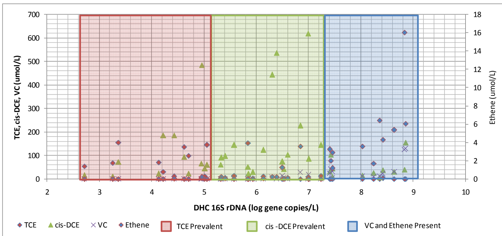
Figure 5-24. Relationship Between TCE and Reductive Daughter Products and Concentrations of DHC 16S rRNA Genes.
