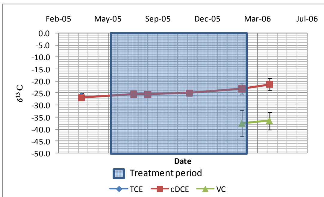
Figure 5-20. Results of CSIA, Values Represent the Mean of All Sampling Points (N=16), Except the April 2006 (N=4), Within Two Treatment Cells and Error Bars Represent One Standard Deviation.
