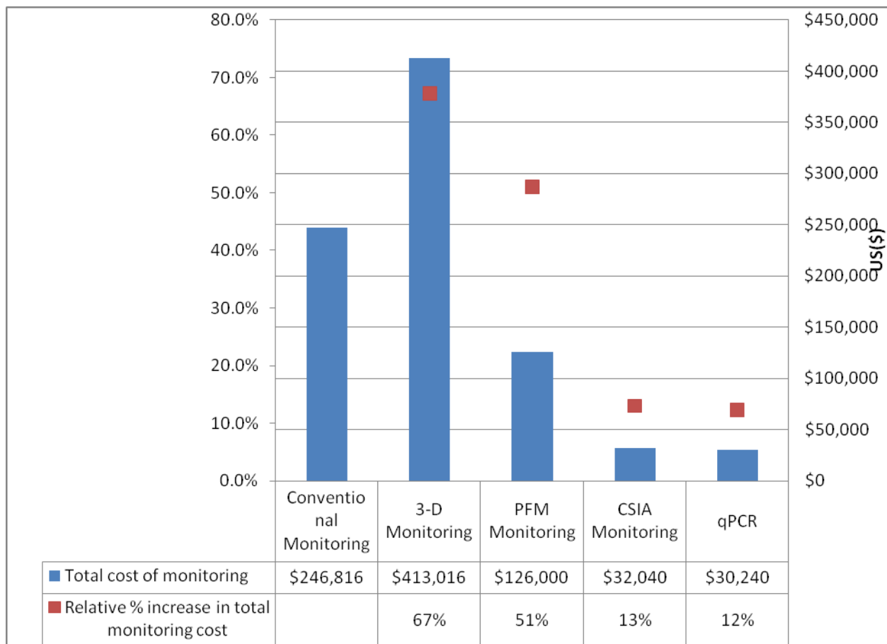
Figure 7-1. Additional Cost for Innovative Diagnostic Tools Included in the Monitoring Strategy Over the Base Case Conventional Monitoring Program.
