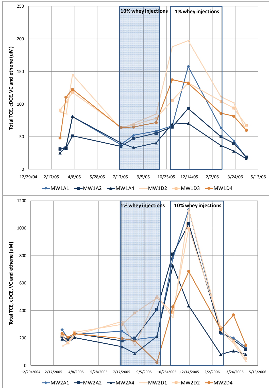
Figure 5-9. Summary of Contaminant Distribution as Total TCE, cDCE, VC, and Ethene in Treatment Cells 1 and 2 Monitoring Wells A and D During Phases 2 and 3.
