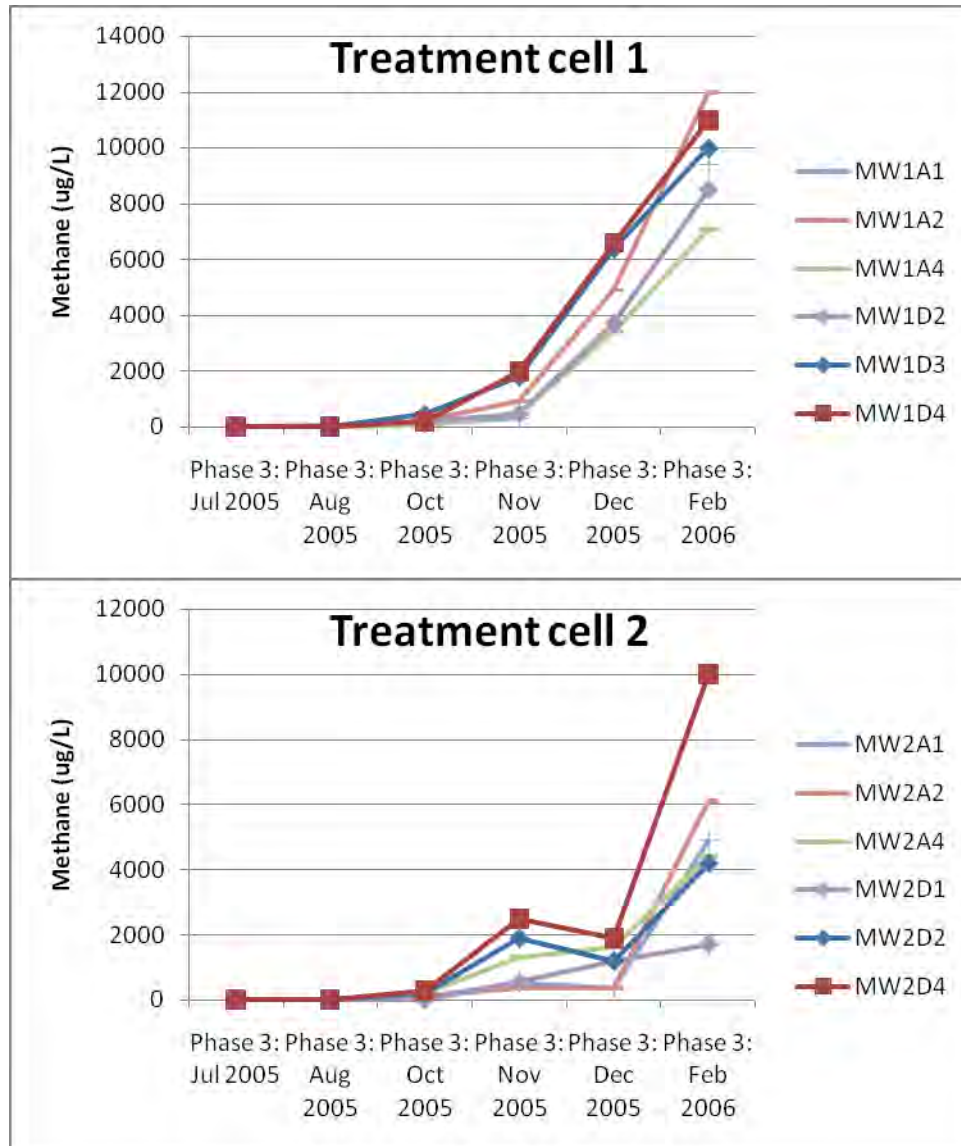
Figure 5-8. Methane Production Observed at Discrete Vertical Depths During Phase 3.
