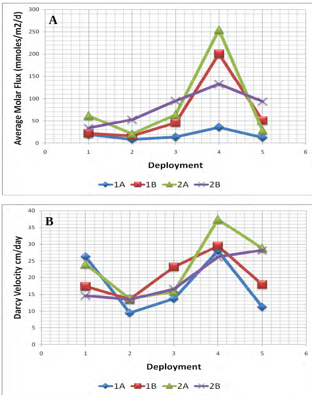
Figure 5-17. Relationship Between Total Average Molar Mass Flux for Each PFM Well for the Five Deployments (A) and Variability in Darcy Velocity (B).
