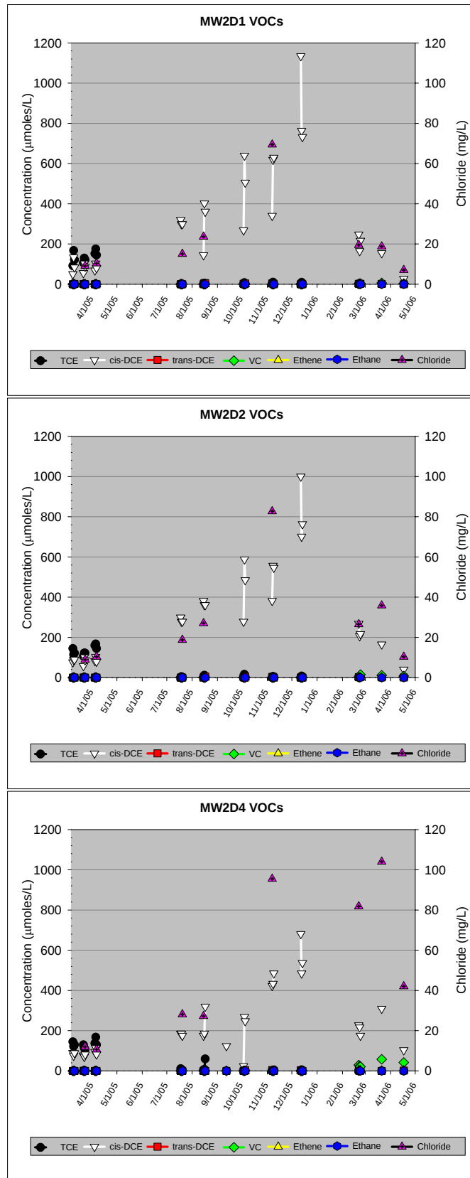
Figure 5-13. Molar Mass Plots of TCE and Reductive Daughter Products During Phases 2 and 3 of the Demonstration at MWD in Treatment Cell 2.
