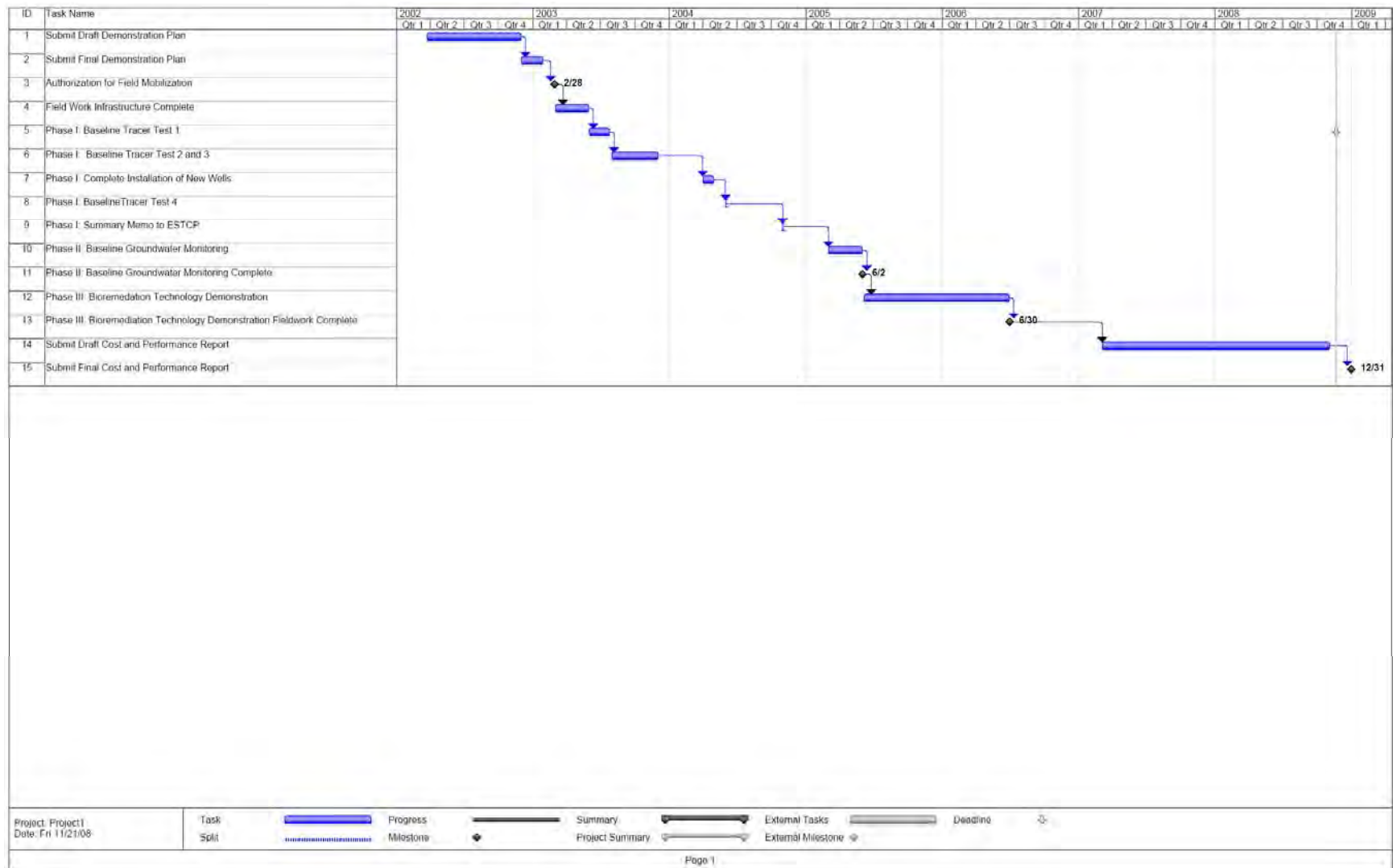
Figure 5-1. Field Schedule for Phases 1, 2, and 3.
