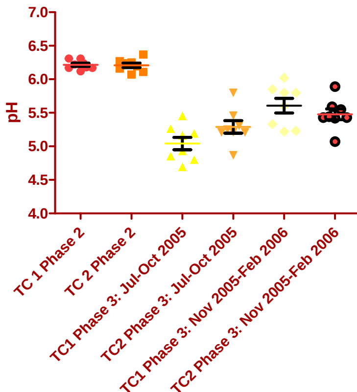
Figure 5-7. Impact of Whey Injection on pH in the Treatment Cells (Lines Represent the Mean and Error Bars Represent One Standard Deviation from the Mean).
