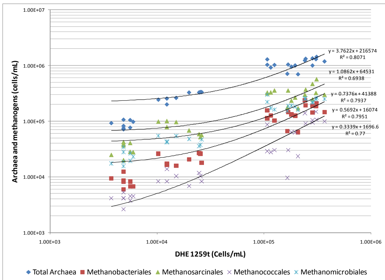
Figure 5-32. Relationship Between Methanogenic Populations and DHC Using FISH During Phase 3 Operations, Values Represent the Mean of N=4 Sampling Points (Port 4 of Each CMT Well) for Each Treatment Cell.
