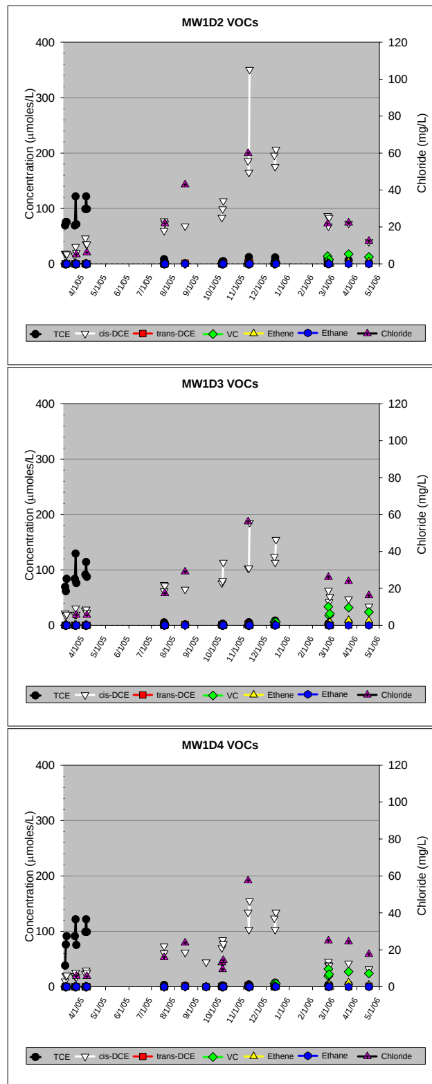
Figure 5-11. Molar Mass Plots of TCE and Reductive Daughter Products During Phases 2 and 3 of the Demonstration at MWD in Treatment Cell 1.
