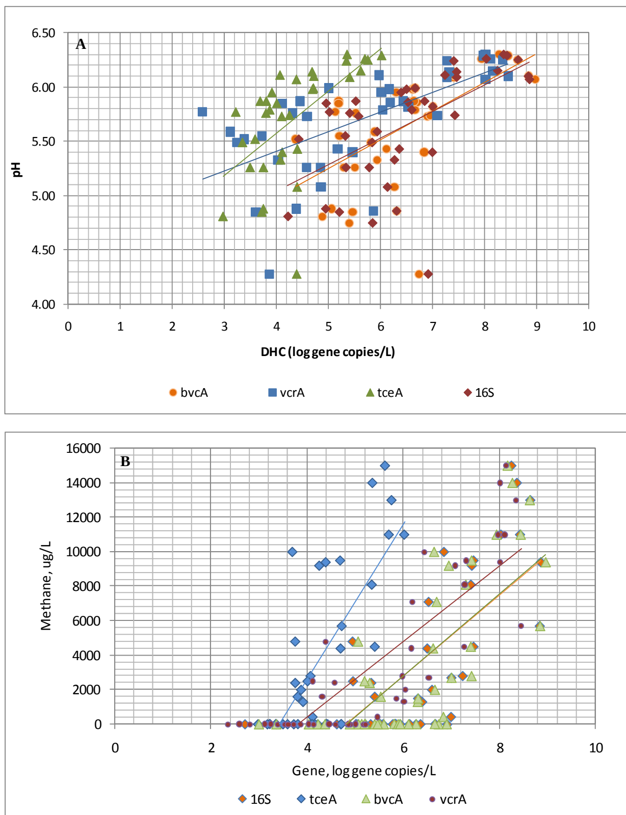
Figure 5-27. Relationship Between DHC qPCR Results and Geochemical Parameters pH (A) and Methane (B).
