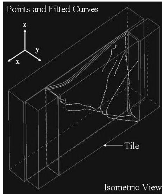
Figure 11. 3-D point cloud and boundary curves of the crack planes.
