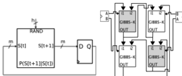
Figure 12 Stochastic digital state machines
