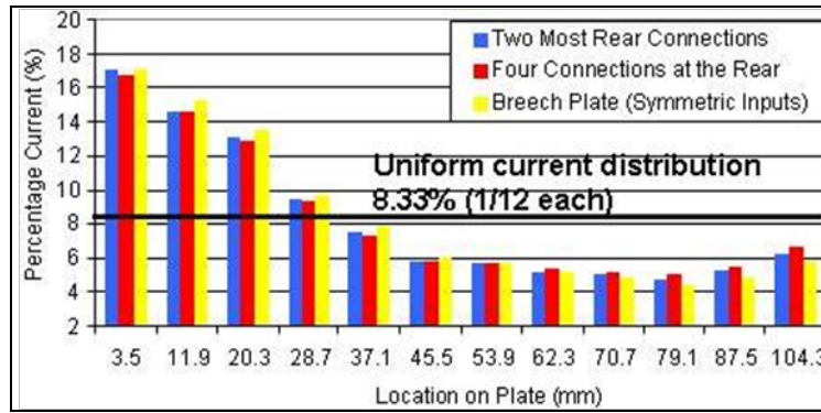
Figure 7. “B-dots” plate current measurement integrated over 1 ms versus plate position.
