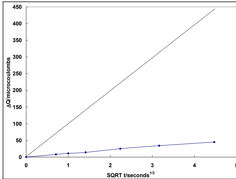
Figure 7. Comparison of decreased hydrogen adsorption charge corresponding to ethanol adsorption ( 10^{-3} \text{ M} solution at 0.3 \text{ V} ) with calculated decrease assuming one hydrogen adsorption site/ethanol molecule adsorbed.
