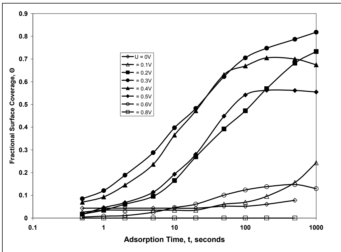
Figure 8. Adsorption of ethanol from a 10^{-3} solution in 1N \text{HClO}_4 .
