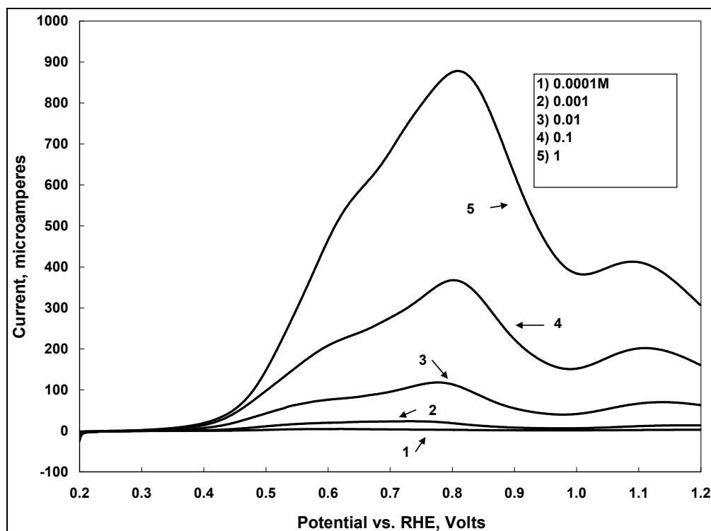
Figure 5. Polarization curves for ethanol oxidation/desorption using the sequence of table 1, v = 1 mv/s.
