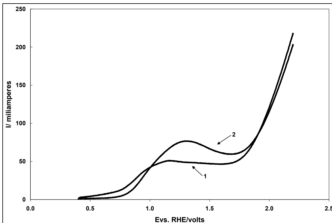
Figure 4. Anodic scans with/without ethanol addition, using the sequence of table 1. Trace 1: 1N \text{HClO}_4 ; Trace 2: 1N \text{HClO}_4 , 10^{-3} M ethanol. V = 200 V/s.
