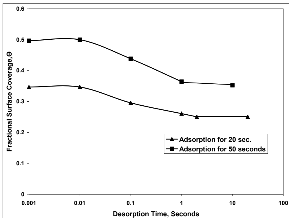
Figure 12. Desorption of ethanol at 0.03 V after adsorption at 0.23 V.
