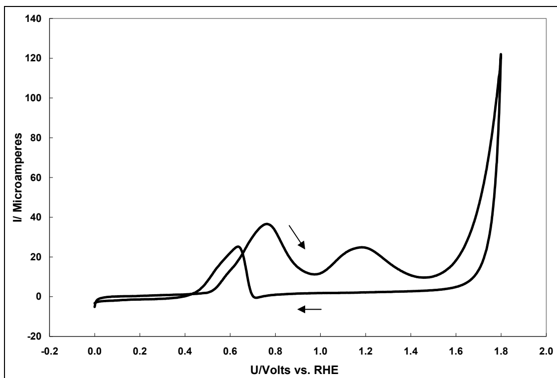
Figure 2. Cyclic voltammogram for 10^{-3} \text{ M} ethanol in 1\text{N HClO}_4 , v = 1 \text{ mv/s} , 10^{-3} \text{ M} ethanol in 1\text{N HClO}_4 .
