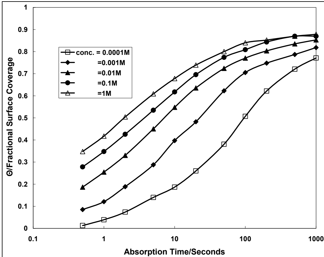
Figure 9. Adsorption of ethanol at 0.3 V.
