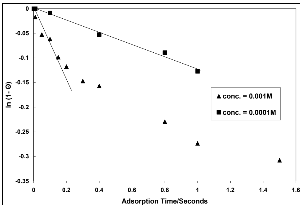
Figure 11. Test of equation 7 for short adsorption times.
