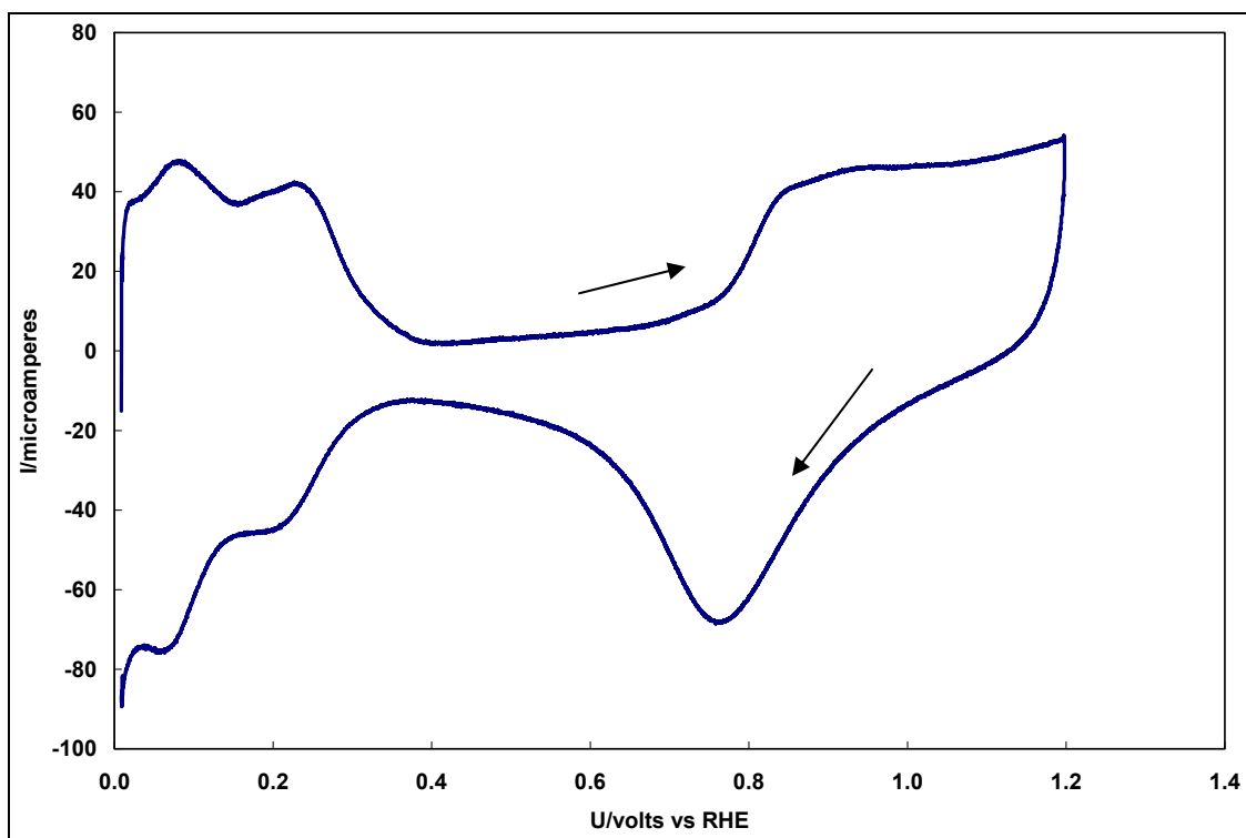
Figure 1. Voltage scan for a 1N solution of \text{HClO}_4 , v = 100 \text{ mv/s} .
