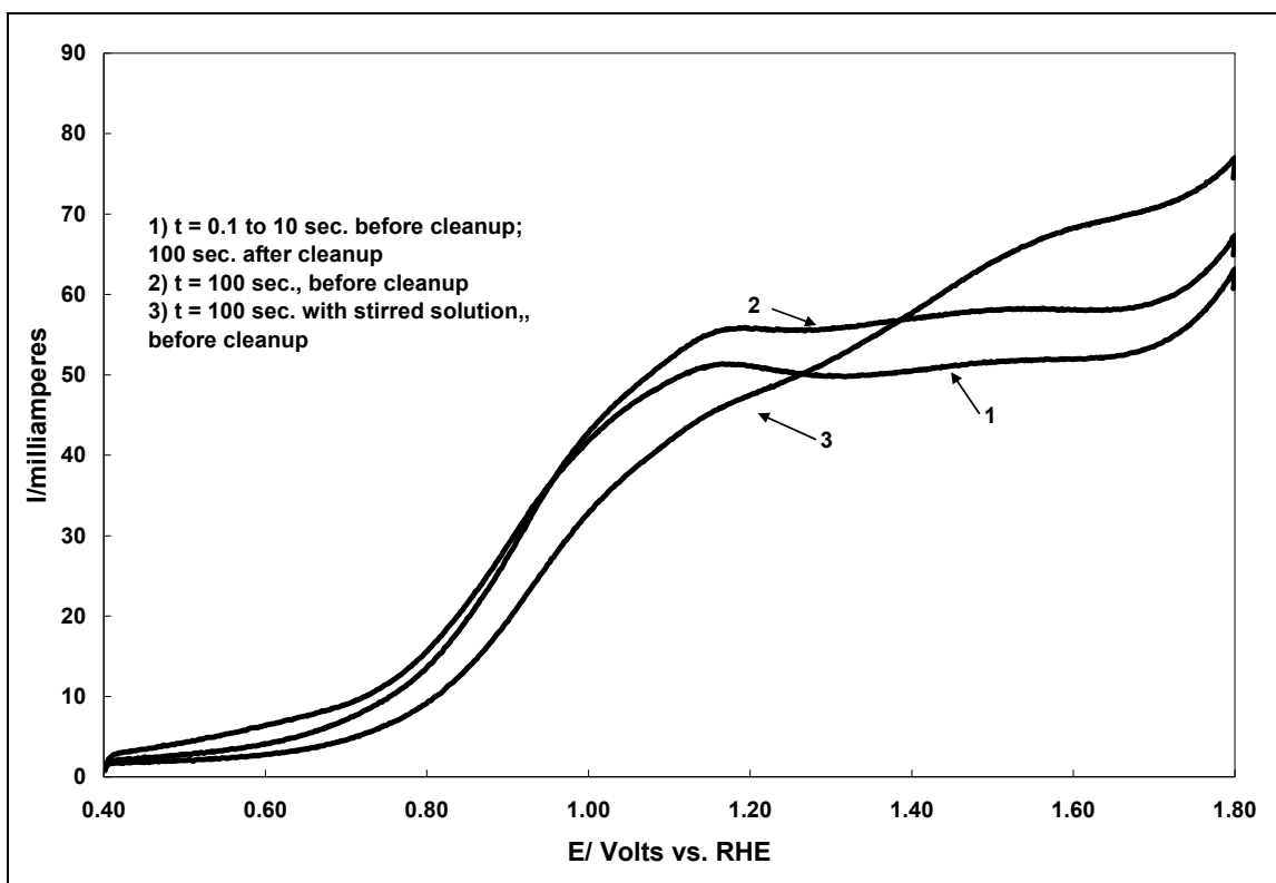
Figure 3. Anodic scans for 1N \text{HClO}_4 using the sequence of table 1, v = 200 V/s.
