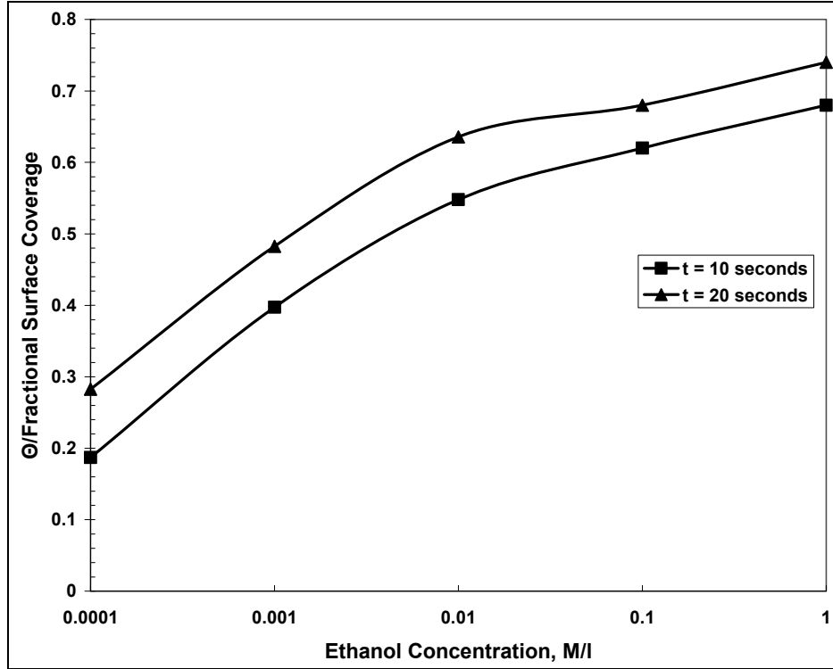
Figure 10. Fractional surface coverage with ethanol at fixed adsorption time.
