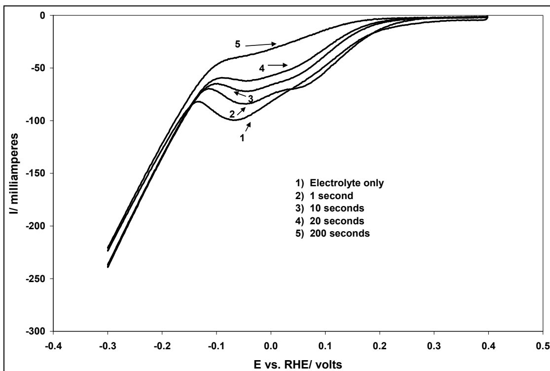
Figure 6. Representative cathodic scans for adsorption of ethanol at open circuit from a 10^{-3} M solution of ethanol in 1N HClO 4 ; potential = 0.3 V, sweep speed = 200 V/s.
