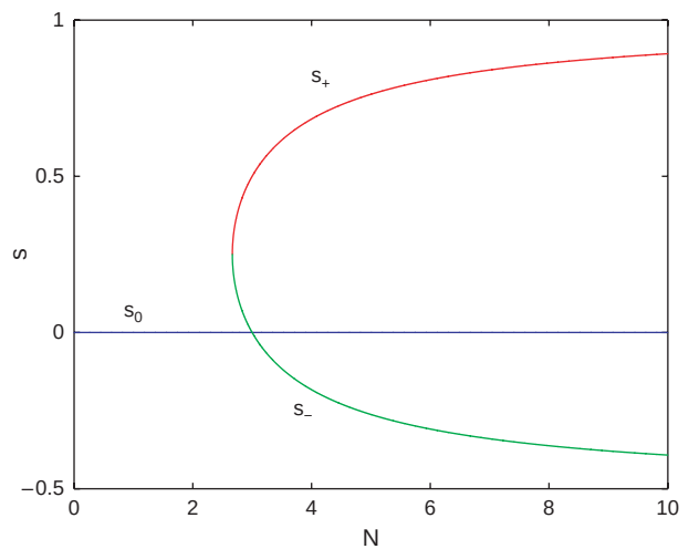
Fig. 3. Isotropic-nematic phase diagram for the Maier-Saupe intermolecular potential with the Doi closure tensor theory. The horizontal axis represents the strength of the nematic potential whereas the vertical axis denotes the nematic order parameter.
