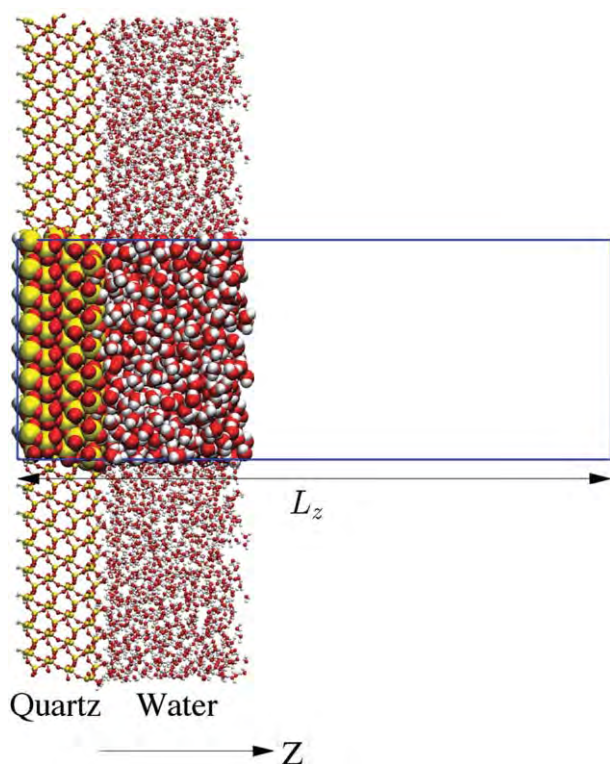
FIG. 1. A snapshot from the simulation of a quartz/water interface embedded in vacuum. The blue box represents the unit simulation cell with a box length in the z -direction ( L_z ) of 100 Å. The simulation cell is repeated periodically in all three directions. Water is in contact with the hydrophilic side of the quartz (011). Empty space (vacuum) is used to separate water and the other side of the quartz crystal in the z -direction.
