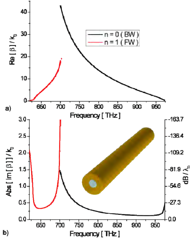
Figure 9 - Dispersion of the real (a) and imaginary (b) part of \beta , normalized to \text{Re}[-ik_b] calculated at the central frequency, for a cylindrical nanorod made of SiC with radius a = 5 \text{ nm} embedded in an unbounded silver background.
