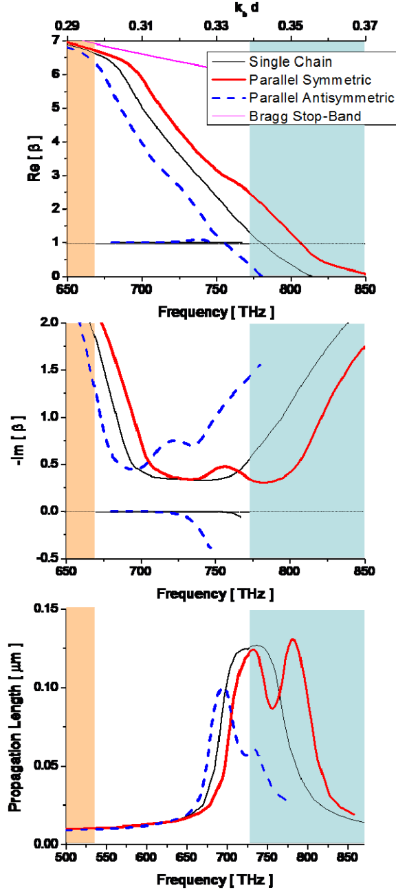
Figure 38 – Similar to Fig. 36, modal dispersion for the quasi- transverse y – polarized modes supported by two parallel chains with interchain distance l = 30 nm .
