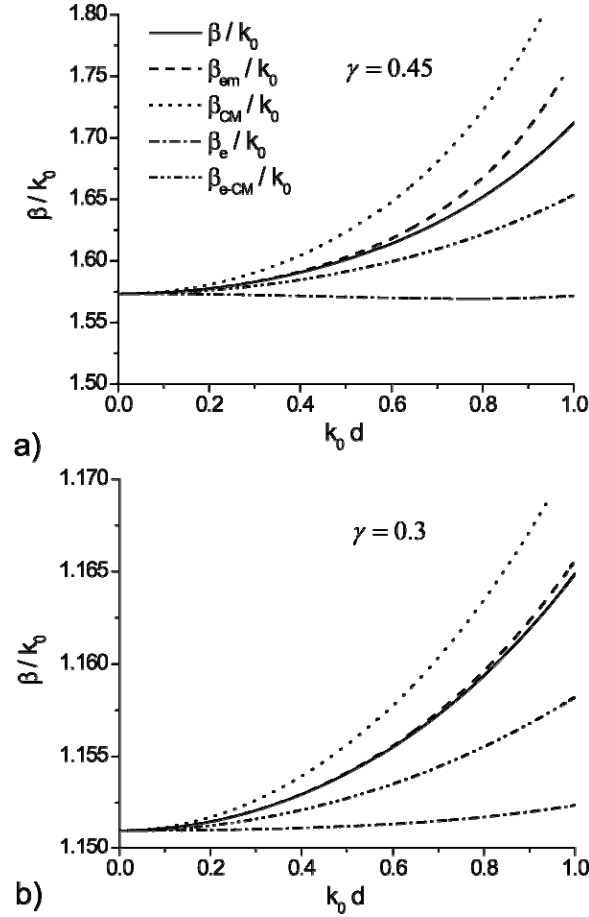
Figure 45 – Frequency dispersion of the guided wave number, and its approximations as defined in the text, for an array of dielectric spheres with \varepsilon = 20 \varepsilon_0 , with (a) \gamma = 0.45 , (b) \gamma = 0.3 .
