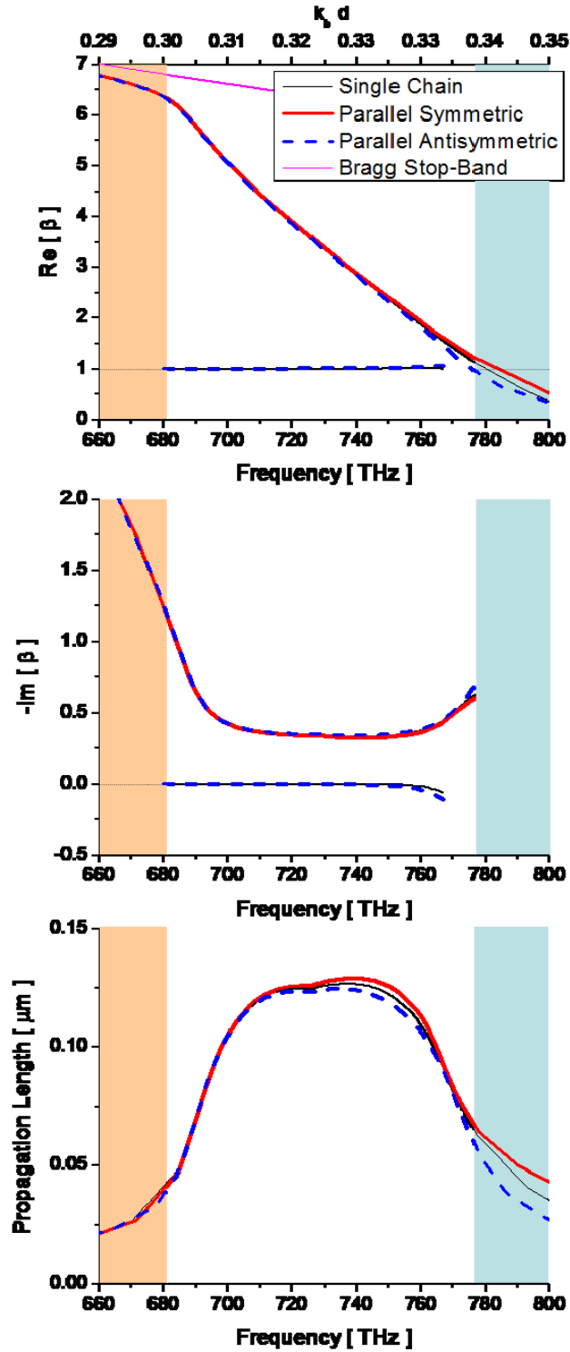
Figure 41 – Analogous to Fig. 31 and Fig. 36, modal dispersion for the quasi- transverse z – polarized modes supported by two parallel chains with interchain distance l = 50 nm .
