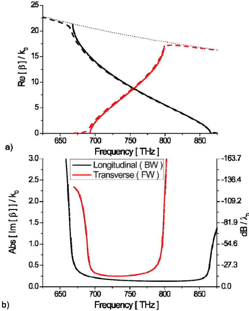
Figure 8 - Dispersion of the real (a) and imaginary (b) part of \beta , normalized to k_0 , for a linear array of SiC voids of radius a = 5\text{nm} in a silver background with d = 10.5\text{nm} . The thin dotted line corresponds to the condition \beta = \pi/d , which is the upper limit for modal propagation, whereas the dashed lines refer to the case in which material losses are neglected.
