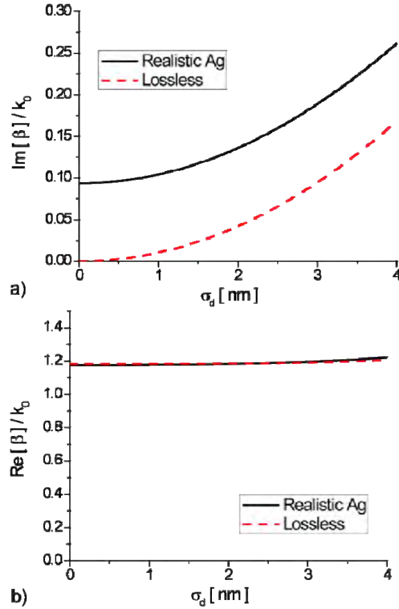
Figure 3 – Similar to Fig. 2, but for a = 15\text{ nm} and average distance d = 33\text{ nm} at the free-space wavelength \lambda_0 = 390\text{ nm} .
