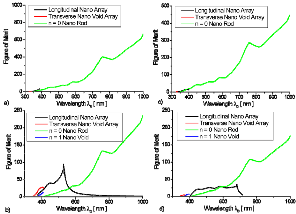
Figure 11 - Figure of merit for the four classes of forward-wave 1D waveguides in Fig. 10 (when available) for four different scenarios: (a) silver and free-space with a = 25\text{ nm} ; (b) silver and silicon-nitride with a = 25\text{ nm} (corresponding to Fig. 10); (c) silver and free-space with a = 5\text{ nm} ; (d) silver and silicon-nitride with a = 5\text{ nm} .
