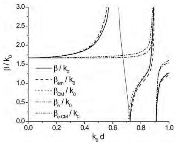
Figure 48 – Frequency dispersion of the guided wave number, and its approximations as defined in the text, for an array of dielectric spheres with \epsilon = 120 \epsilon_0 and \gamma = 0.45 . The thin solid line corresponds to the imaginary branch of \beta .
