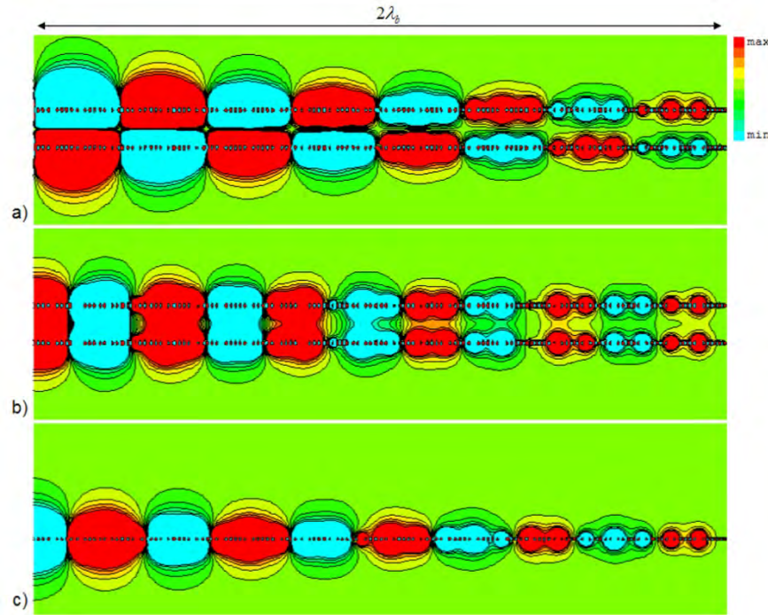
Figure 43 – (Color online). Electric field distribution (snapshot in time) for the chains of Fig. 41 at frequency f = 750 \text{ THz} . (a) antisymmetric mode, (b) symmetric mode, (c) isolated chain.
