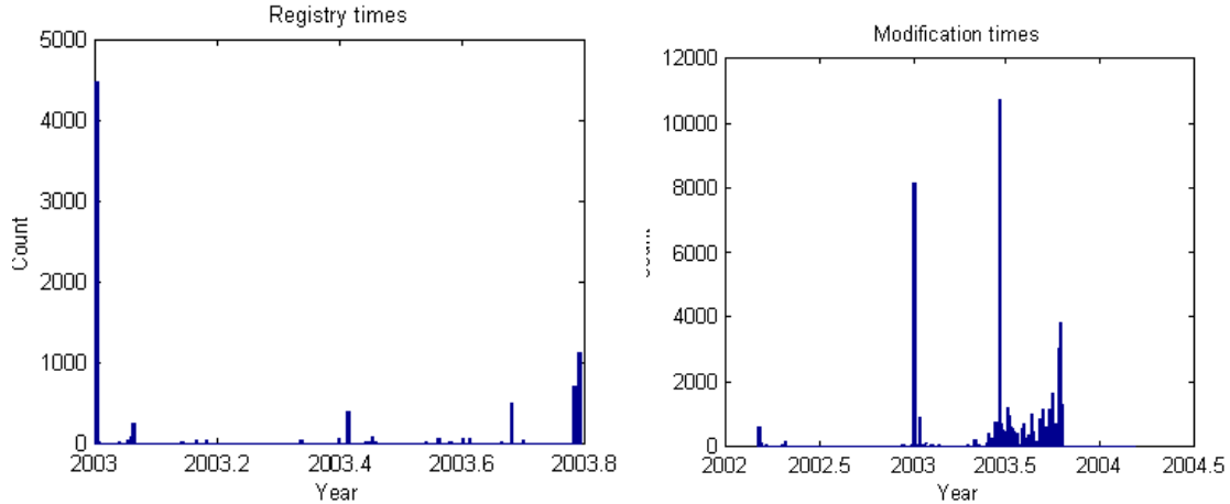
Figure 7: Registry times versus file modification times for an example disk.
