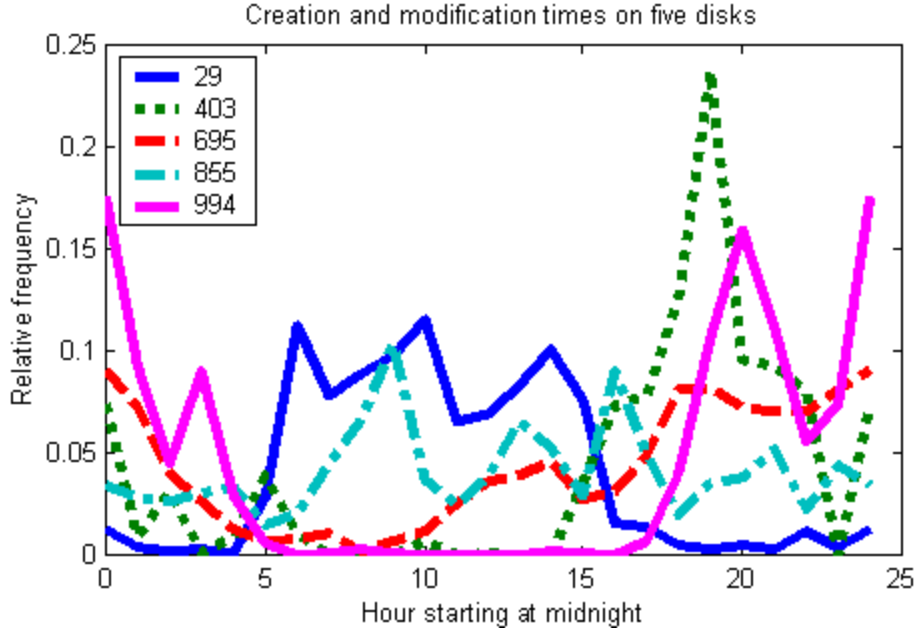
Figure 6: Usage per hour of five disks.
