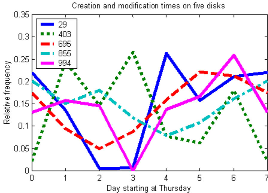
Figure 5: Usage per day of five disks.
