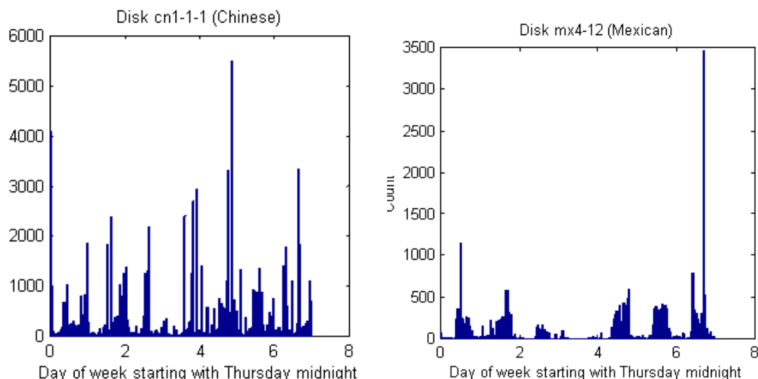
Figure 3: Histograms of modification times in week for two example disks.
