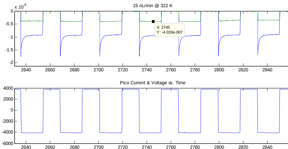
Figure 28: Negative Current
