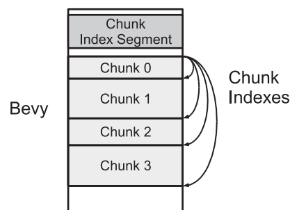
Fig. 4 – The structure of Image Stream Bevy. Each bevy is a collection of compressed chunks stored back to back. Relative chunk offsets are stored in the chunk index segment.
