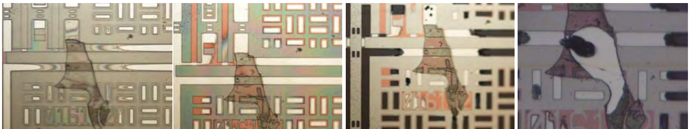
Figure 9: 'tent-pole' imprint defect results in tenting, micromasking and delamination. The evolution of the defect through the SAIL process starts at the left following the imprint, through the successive etch processes and finally adhesion and tearout on the right.
