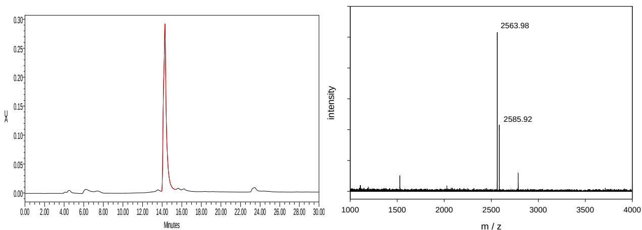
Fig. 14. Characterization of AlexaFluor 532-GE11. Left: analytical reversed phase liquid chromatography of purified agent by a 30 min gradient from 20% to 75% CH 3 CN in aqueous 0.1% CF 3 CO 2 H, at 1 mL/min, on 4.5 × 250 mm C 18 column, at rt, detected at 260 nm. Right: MALDI-TOF mass spectroscopy after chromatographic purification. The purified main peak was excited from an \alpha -cyano-hydroxycinnamic acid matrix, showing the predicted mass of 2563.98Da (M+H).
