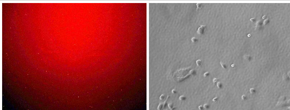
Fig. 21. Internalization of AlexaFluor647-EGF2031 binding to AsPC1 cells for 5 hr at 37°C, recorded on a Zeiss 510 Meta confocal microscope with a 40x/1.3 oil DIC objective. Excitation: 532 nm. Emission: 554 nm. Left: fluorescent image. Right: bright field.
