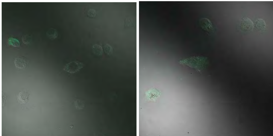
Fig. 20. Internalization of AlexaFluor488-EGF3248 binding to AsPC1 cells for 1 hr at 37°C, recorded on a Zeiss 510 Meta confocal microscope with a 40x/1.3 oil DIC objective. Excitation: 488 nm. Emission: 505-550 nm. Left: 50 nM. Right: 1.0 \mu M.
