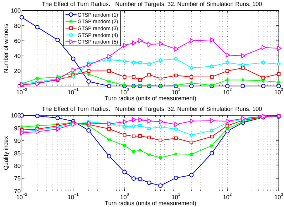
Figure 18. Comparison of GTSP random algorithm with different numbers of angles. When the algorithms do not run to completion, the GTSP algorithm with fewer angle choices outperform when the radius is small.
