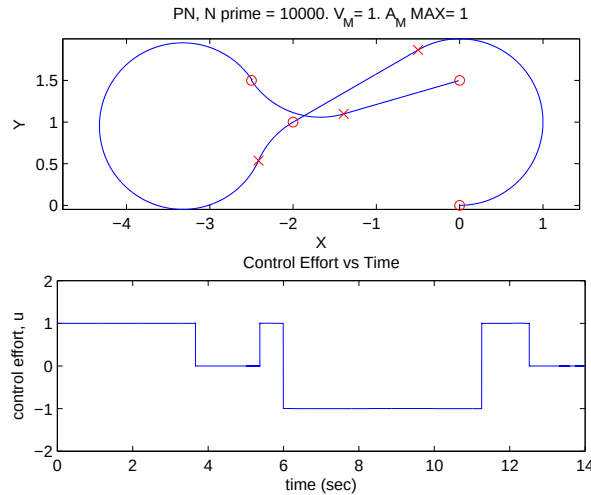
Figure 29. Result for traversing from the origin to 3 targets marked as circles. The navigation constant is very large ( N' = 10000 ). The 'x' marks locations in which there is a fundamental change in control effort.
