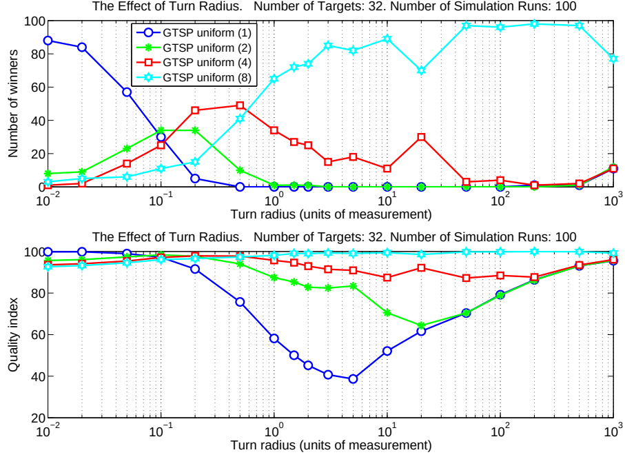
Figure 17. Comparison of GTSP uniform algorithm with different numbers of angles. When the algorithms do not run to completion, the GTSP algorithm with fewer angle choices outperform when the radius is small.
