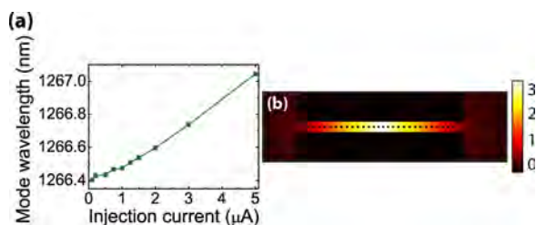
FIG. 4. (Color online) (a) Plot of the cavity peak wavelength versus injection current. (b) 2D map of the change in temperature (in \Delta K ) of the nanobeam device for a bias voltage of 1.2 V. The cavity center only heats by about 3.3 K.
