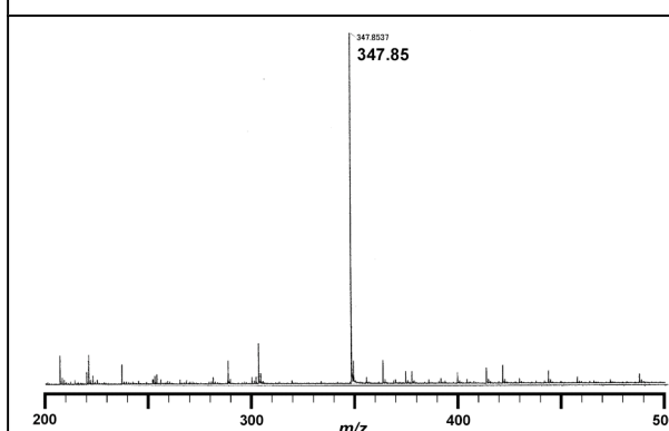
Figure 12. ESI mass spectrum (positive mode) of the preparative peak at 12.2 min in the HPLC analysis of the enzymatic reaction. Exact mass is 347.06 for [\text{dT}^*\text{MP} + \text{H}]^+ .
