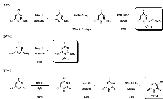
Scheme 4. Synthesis of X^{P*} -I, D^{P*} -I, and T^{P*} -I.
