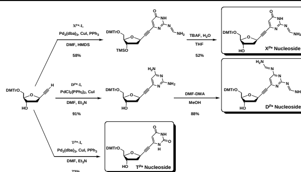
Scheme 5. Synthesis of X^{P*} , D^{P*} , and T^{P*} nucleosides.
