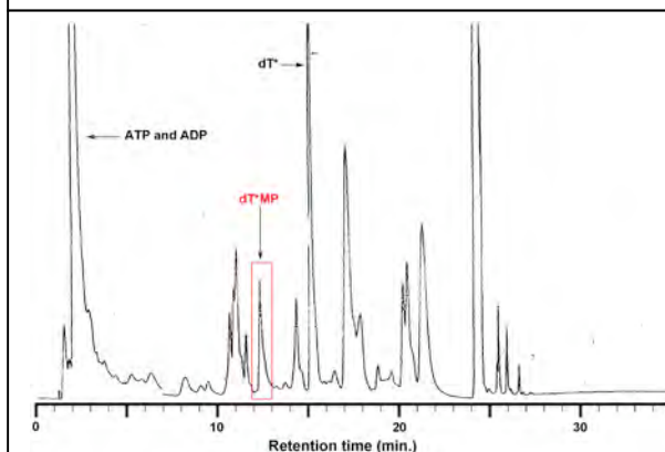
Figure 11. An HPLC chart for TK1 enzymatic reaction of T* nucleoside after 18 h.
