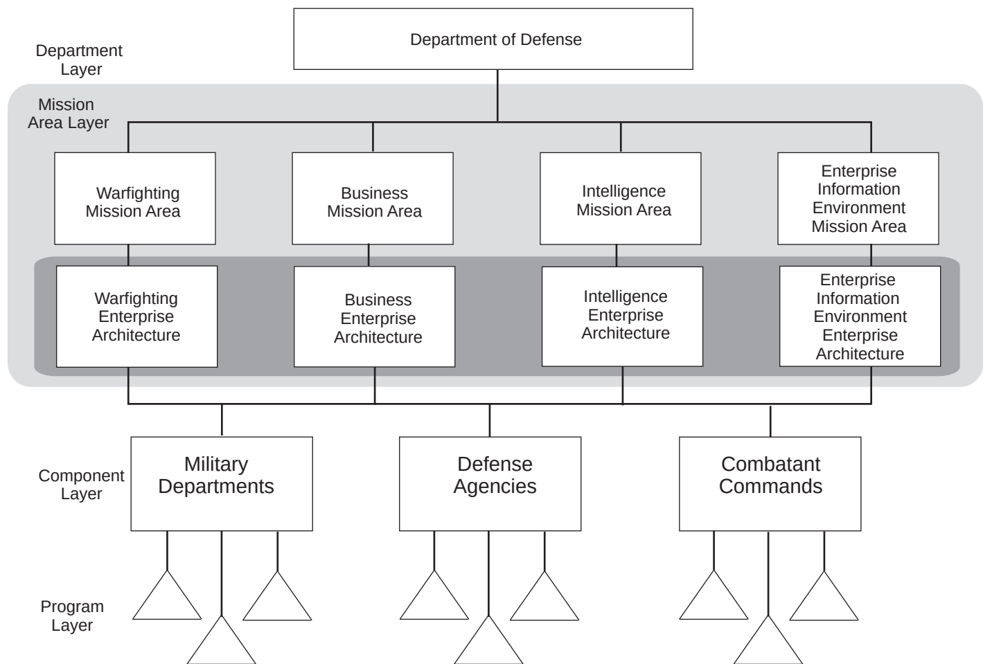
Figure 2: Conceptual Representation of DOD's Federated Architecture
