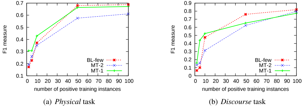
Figure 1: The effect of the amount of training data on the performance.
