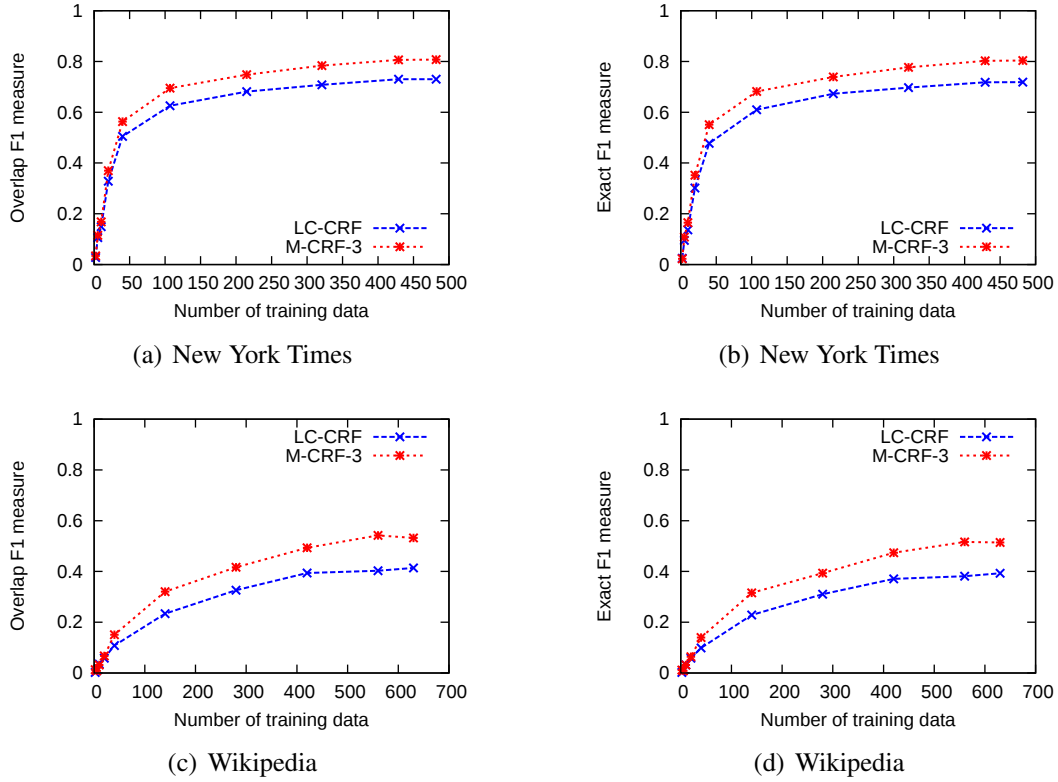
Figure 2: The effect of the training data size
