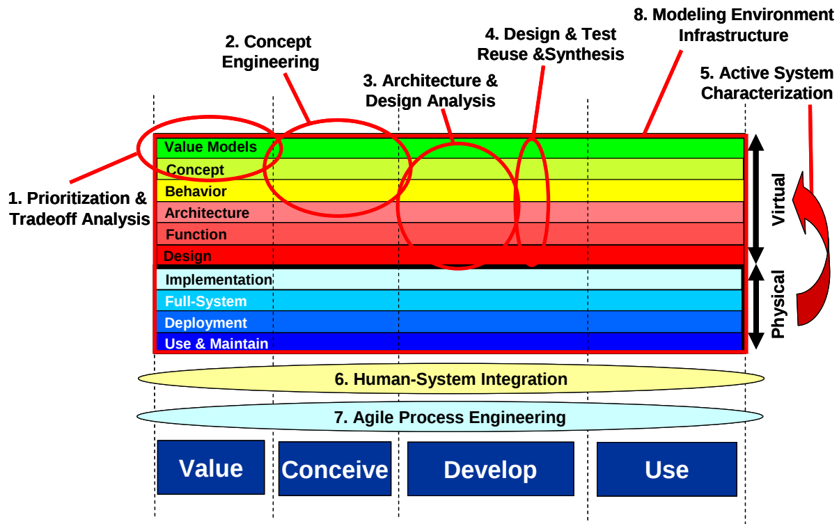
Figure 13: Relationship of SET Research Areas to Modeling Levels
