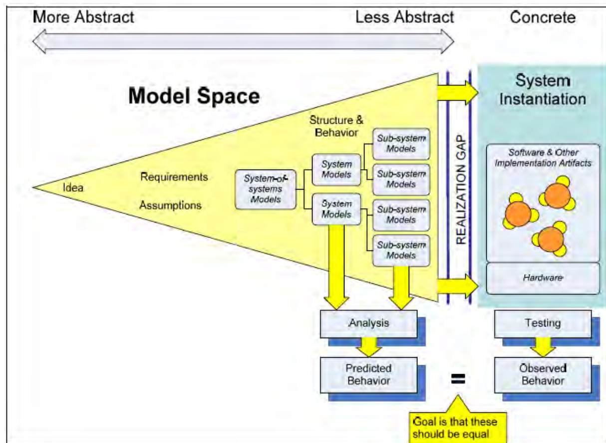
Figure 8: Visualization of System Models (Source: [Watson, 2009])
