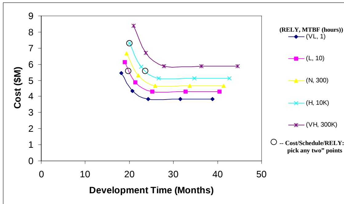
Figure 17: COCOMO II Cost/SCED/RELY Tradeoff Curves, 100K SLOC Project
