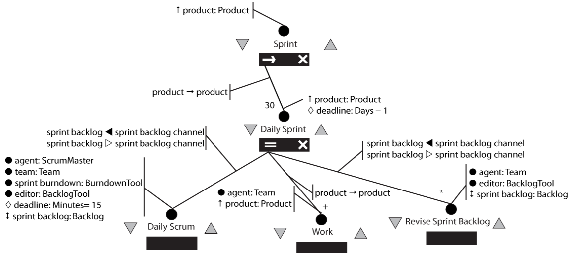
Figure 5: Elaboration of the Sprint step (Source: [Turner, 2007b])
