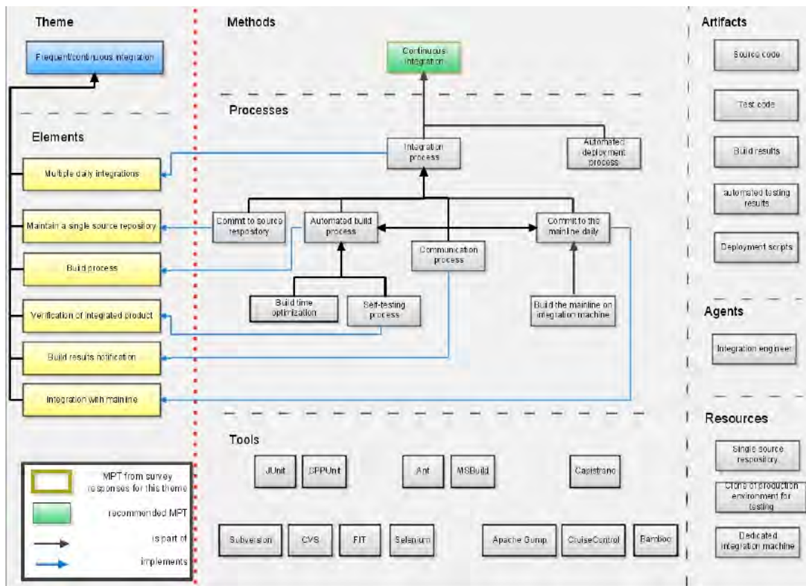
Figure 4: Bridge Diagram for Continuous Integration (Source: [Turner, 2009b])
