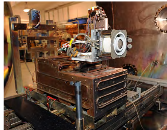
(b) The null-type inverted pendulum thrust stand used for performance measurements.
