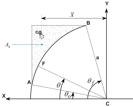
Fig. 4. Area subtended by gate arc AB (shaded)
