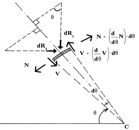
Fig. 6. Free-body diagram of gate differential element
