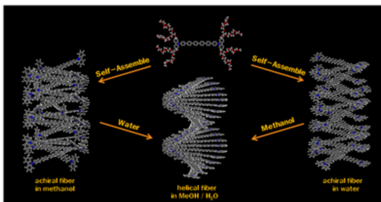
Fig. 3 Schematic representation of the reversible transformation from achiral to chiral states of the cylindrical stack in mixture of methanol and water.
