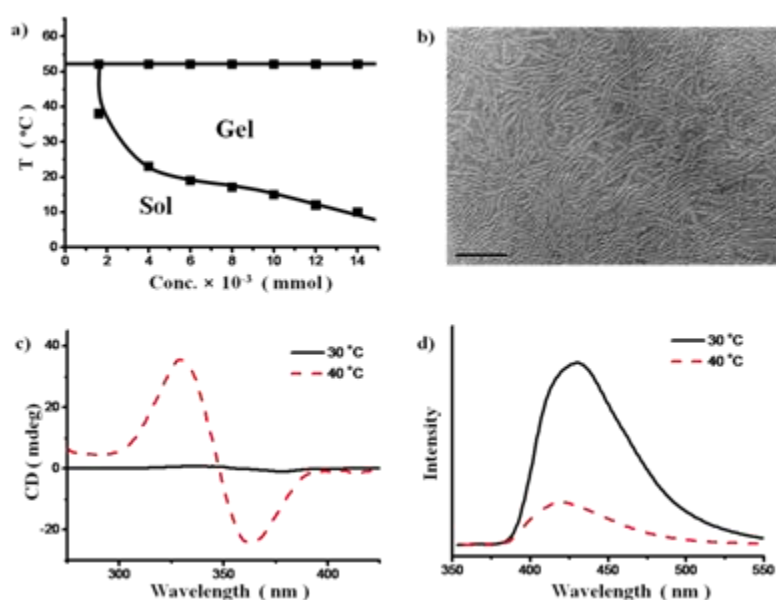
Fig. 4 a) Phase diagram plotted in terms of the concentration of 1 versus temperature. b) TEM images (negatively stained with uranyl acetate) of 1 in aqueous solution prepared at 40 °C ( 1.6 \times 10^{-3} M, scale bars: 100 nm). c) CD spectra of 1 in aqueous solution with 1 mm cell ( 1.6 \times 10^{-3} M). d) Emission spectra of 1 in aqueous solution ( 1 \times 10^{-3} M) at 30 °C (black) and 40 °C (red).
