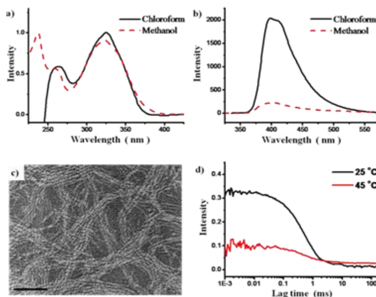
Fig. 1 a) Absorption spectra of 1 in chloroform ( 2.0 \times 10^{-5} M, black), methanol ( 2.0 \times 10^{-5} M, red). b) Emission spectra of 1 in chloroform ( 2 \times 10^{-5} M, black), methanol ( 2 \times 10^{-5} M, red). c) TEM images of 1 methanol solution prepared at 25 °C ( 4 \times 10^{-4} M, scale bars: 50 nm). d) Autocorrelation functions of 1 in methanol ( 4 \times 10^{-4} M) at 25 °C (black) and at 45 °C (red).
