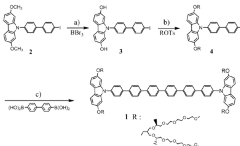
Scheme 1. Synthesis of the end-capped rod amphiphile 1 . a) dichloromethane; b) K_2CO_3 , acetonitrile, reflux; c) Na_2CO_3 , [Pd(PPh_3)_4] , THF, reflux.
