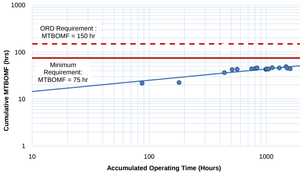
Figure 4. Duane Plot of RMS Test Data Since 2005
