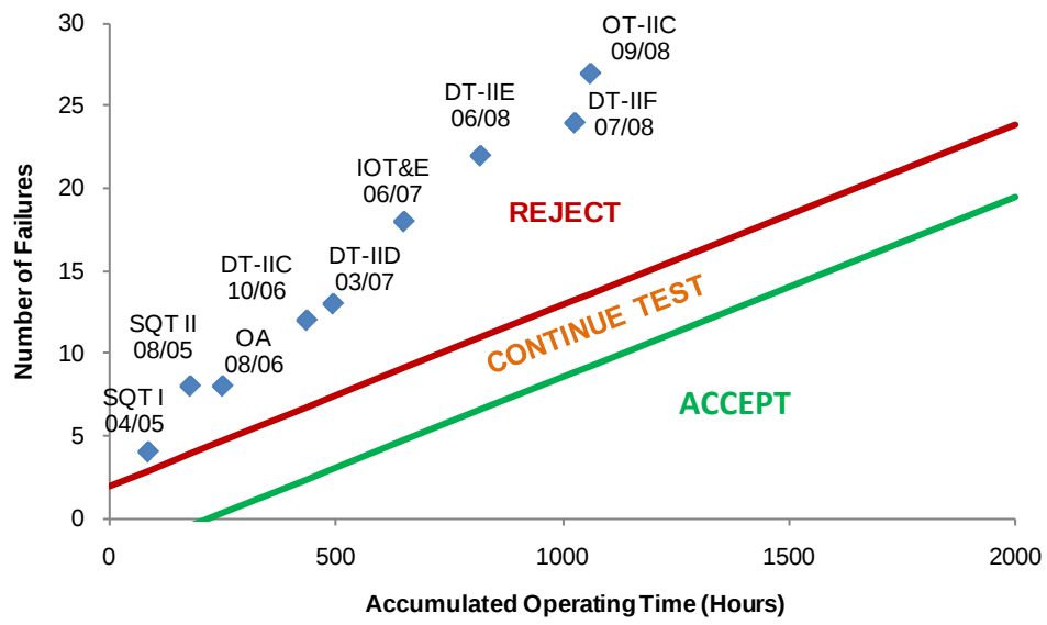
Figure B-1. Probability Ratio Sequential Test Results
