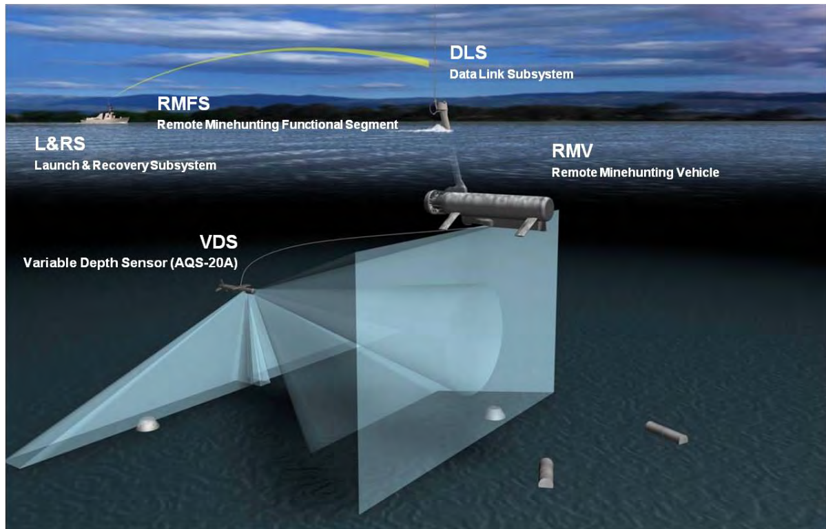
Figure 1. The Five Major Subsystems of the Remote Minehunting System
